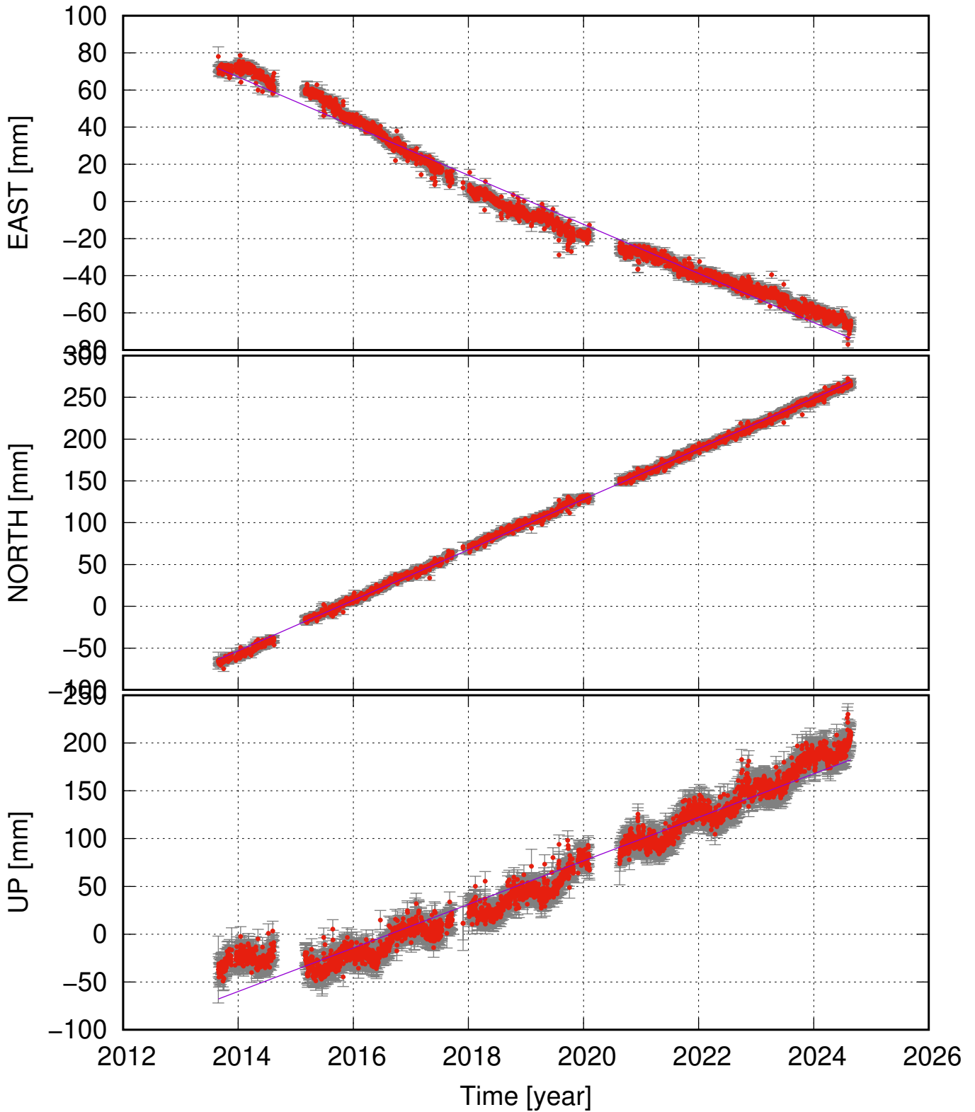
VONC (64.67, -17.75) time series (ITRF 2014) v_e = -13.22 \pm 0.50 ; v_n = 30.21 \pm 0.28 ; v_u = 22.76 \pm 1.38 mm/yr
