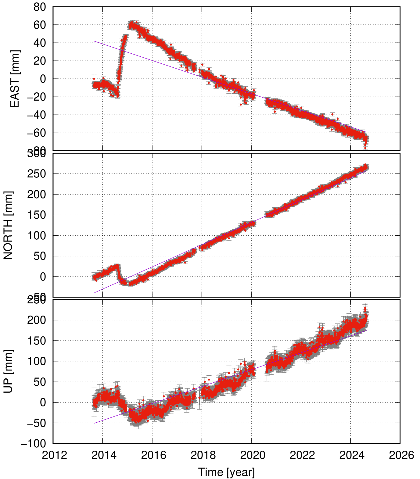
VONC (64.67, -17.75) time series (ITRF 2014) v_e = -9.21 \pm 1.68 ; v_n = 27.00 \pm 1.31 ; v_u = 20.51 \pm 2.10 mm/yr
