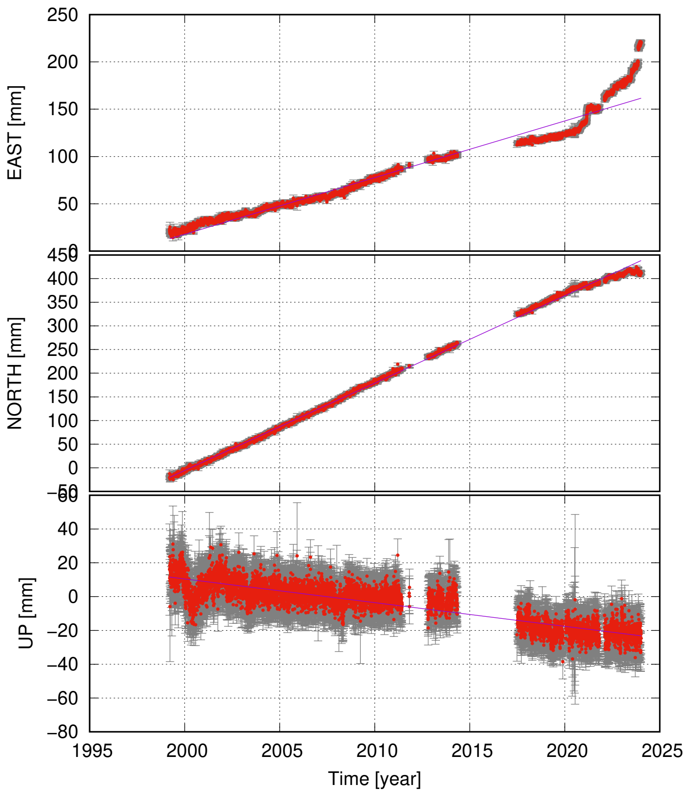
VOGS (63.85, -21.70) time series (ITRF 2014) v_e = 5.99 \pm 0.43 ; v_n = 18.49 \pm 0.21 ; v_u = -1.40 \pm 0.24 mm/yr
