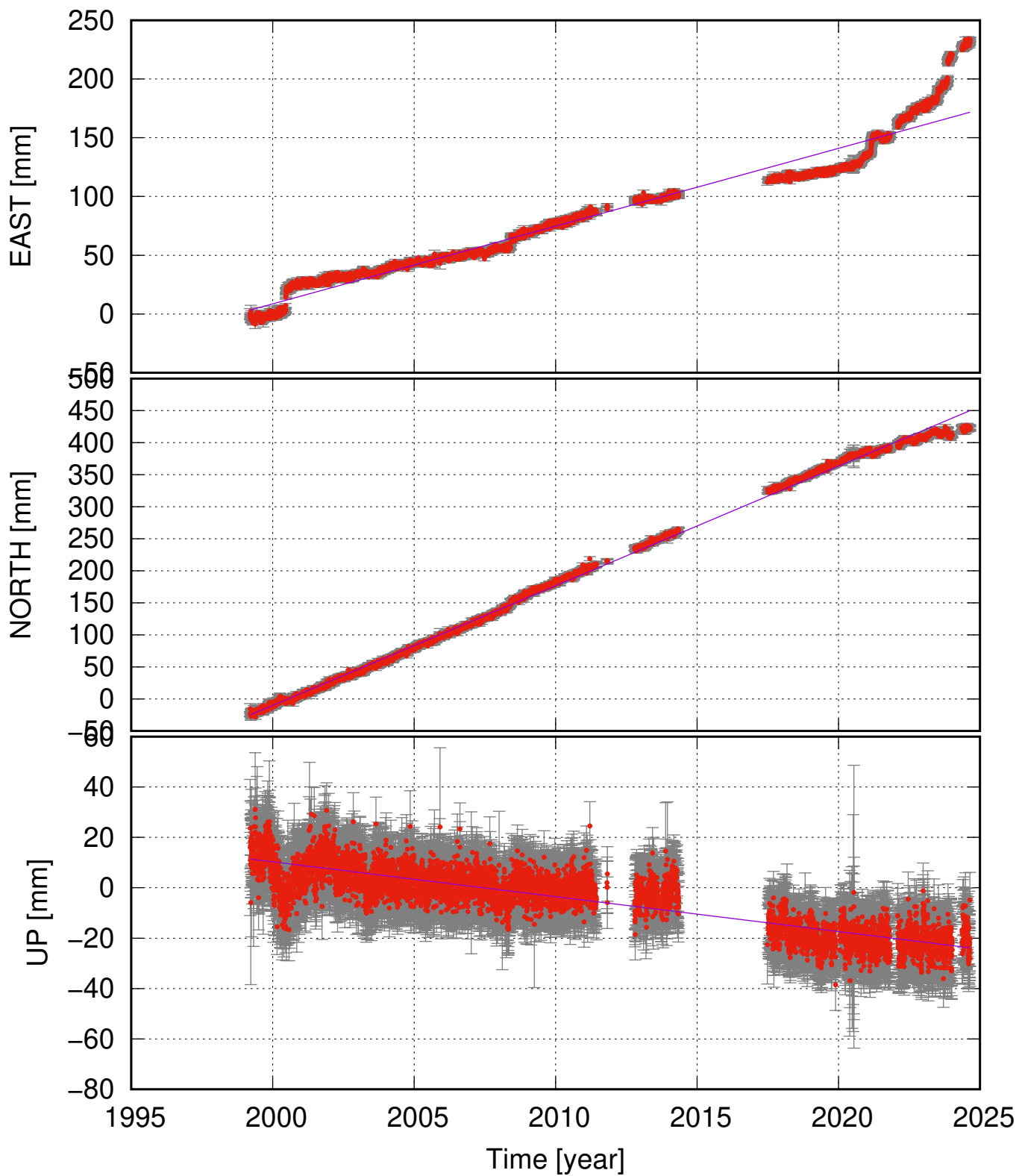
VOGS (63.85, -21.70) time series (ITRF 2014) ve = 6.62 +- 0.50; vn = 18.67 +- 0.26; vu = -1.39 +- 0.23 mm/yr
