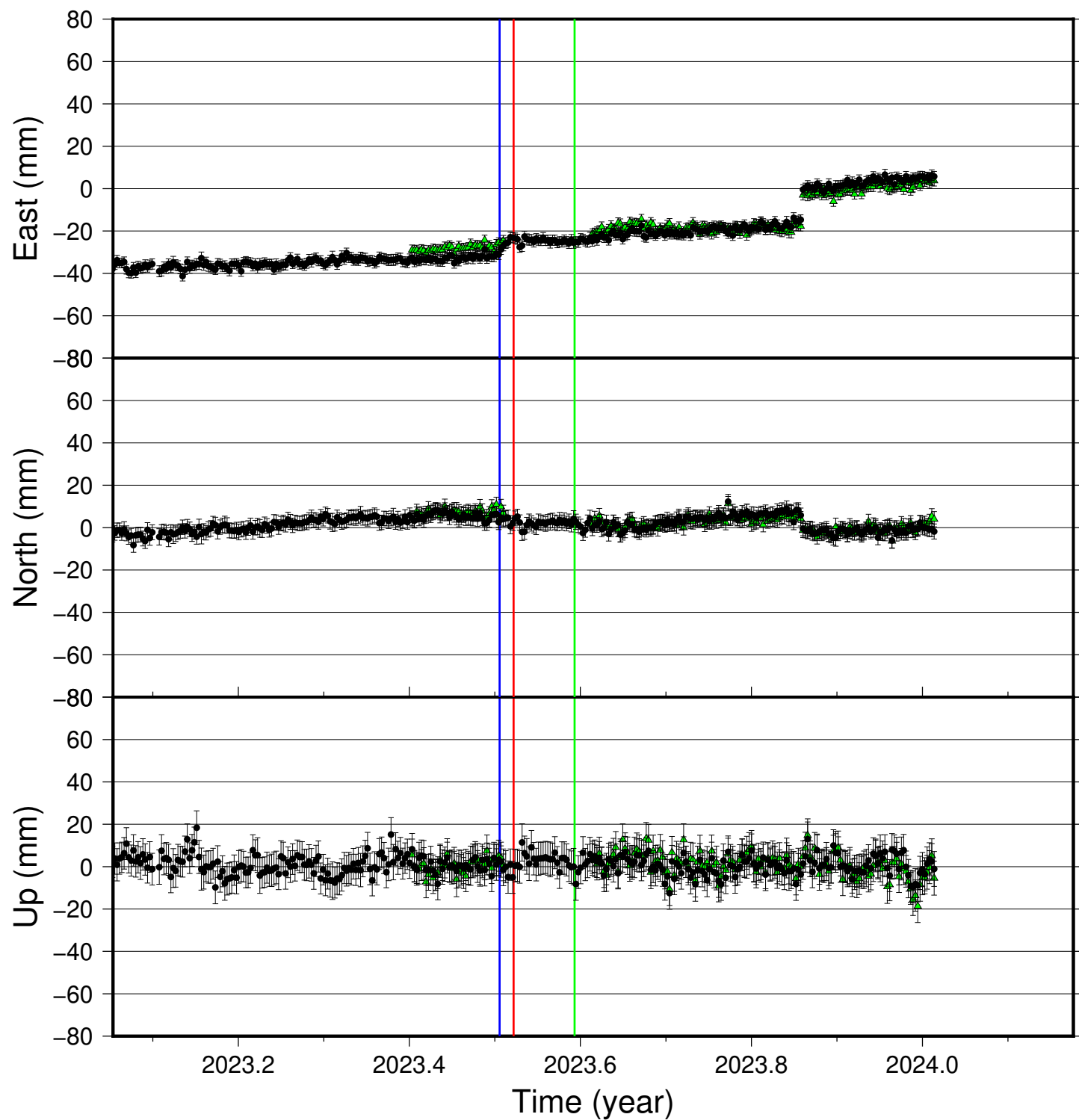
VOGS time series (IGS 2014), last 400 days
