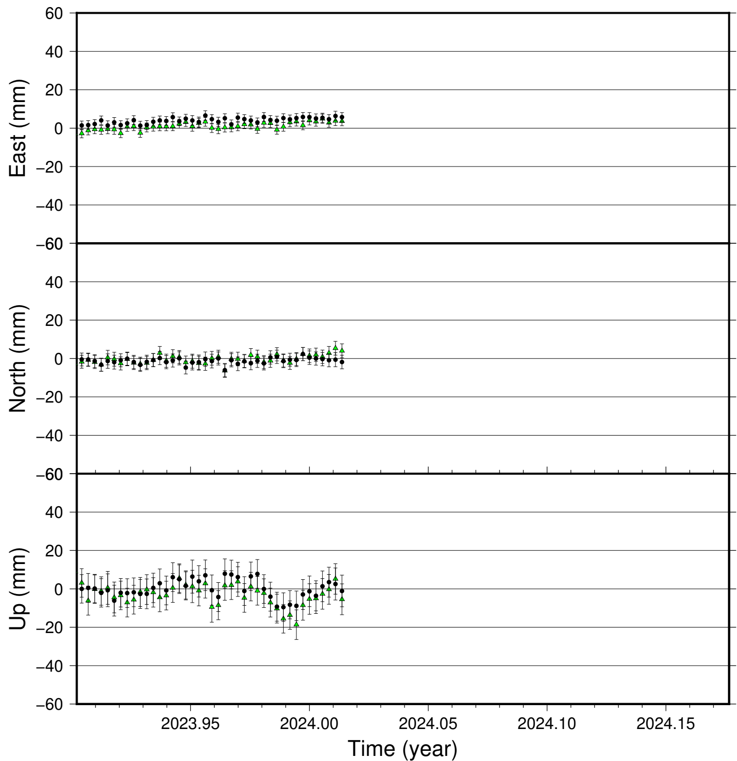
VOGS time series (IGS 2014), last 100 days
