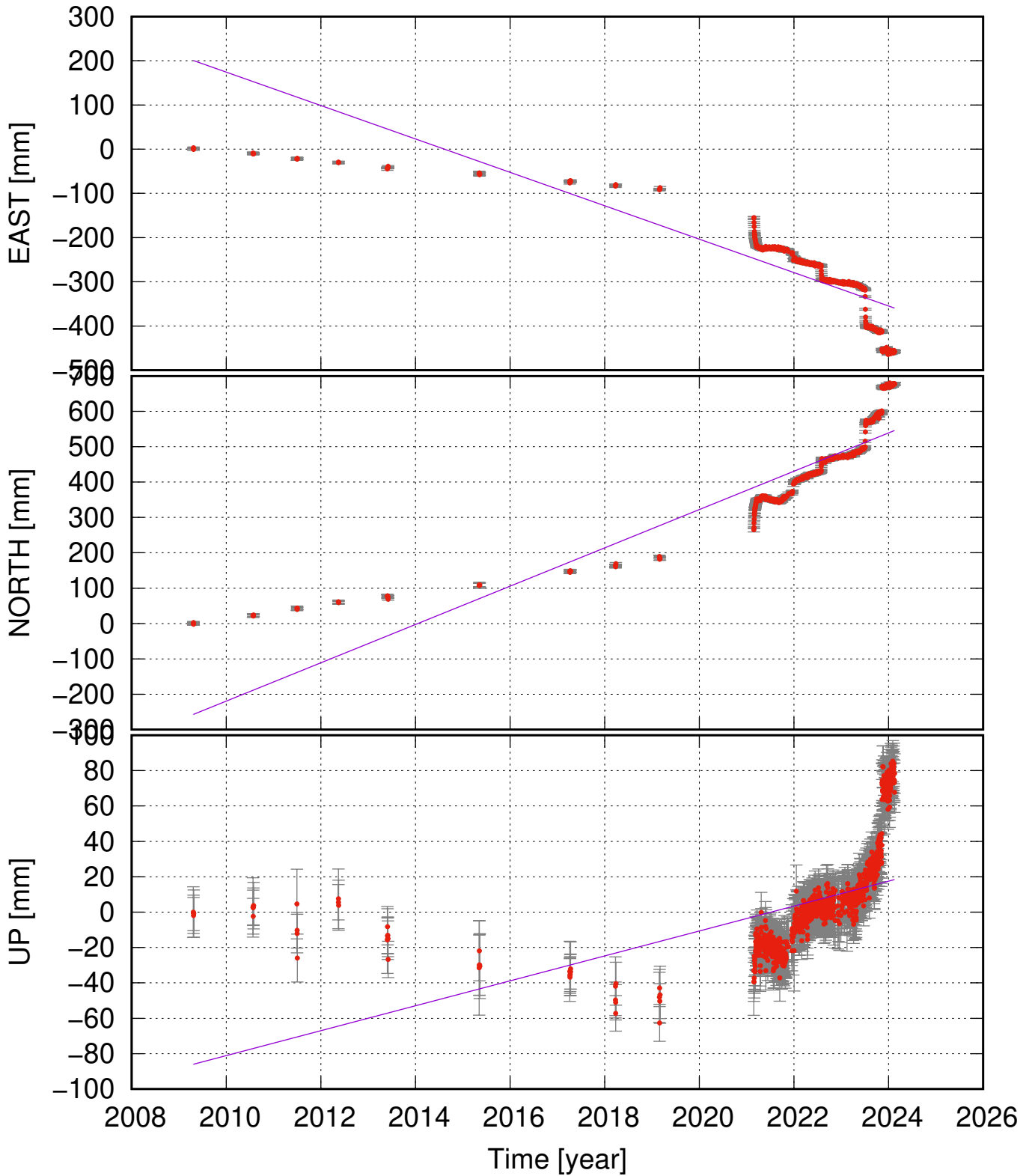
VOGC (63.98, -22.33) time series (ITRF 2014) ve = -37.77 \pm 3.57 ; vn = 54.17 \pm 4.35 ; vu = 7.04 \pm 1.65 mm/yr
