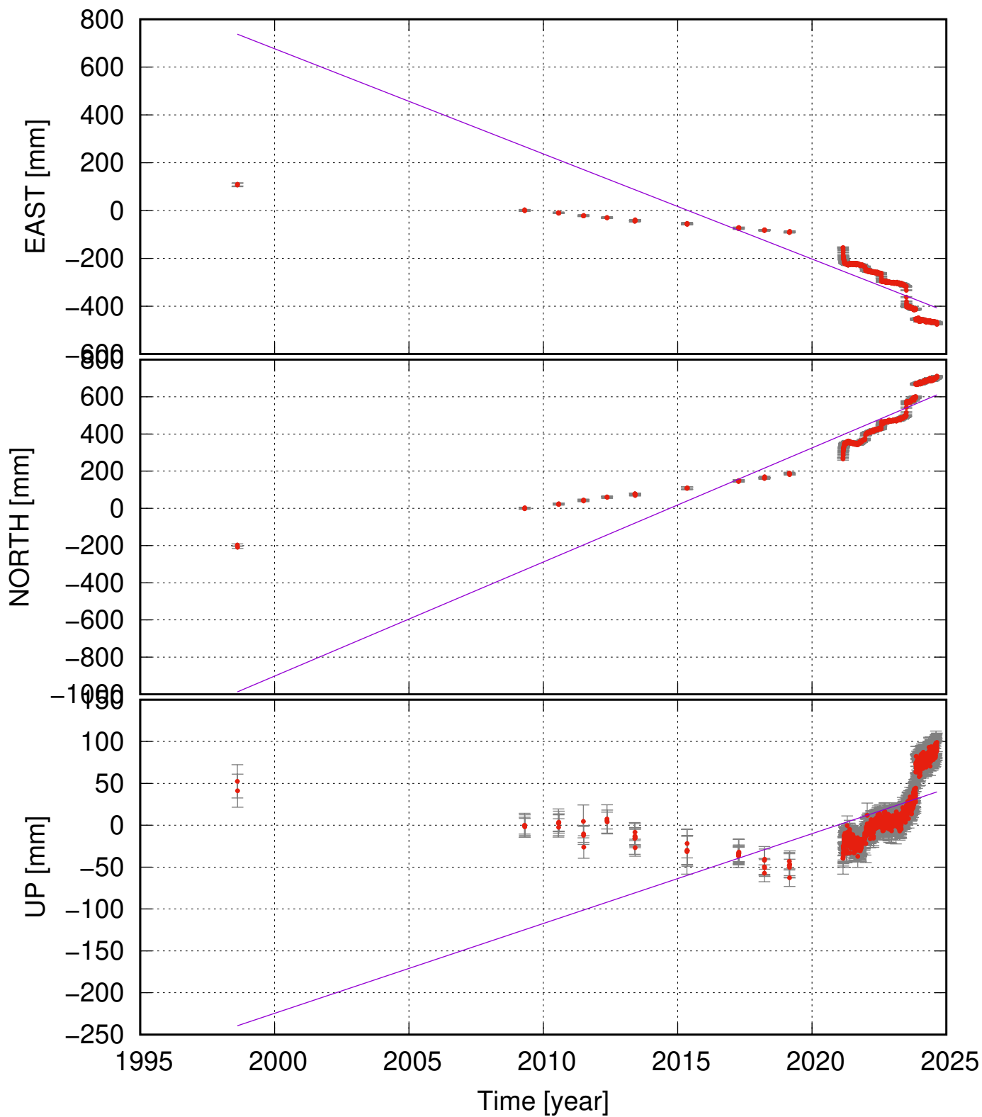
VOGC (63.98, -22.33) time series (ITRF 2014) ve = -43.97 ± 2.45; vn = 61.33 ± 3.10; vu = 10.73 ± 1.29 mm/yr
