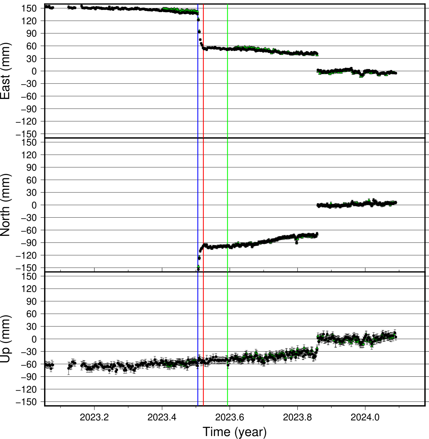
VOGC time series (IGS 2014), last 400 days
