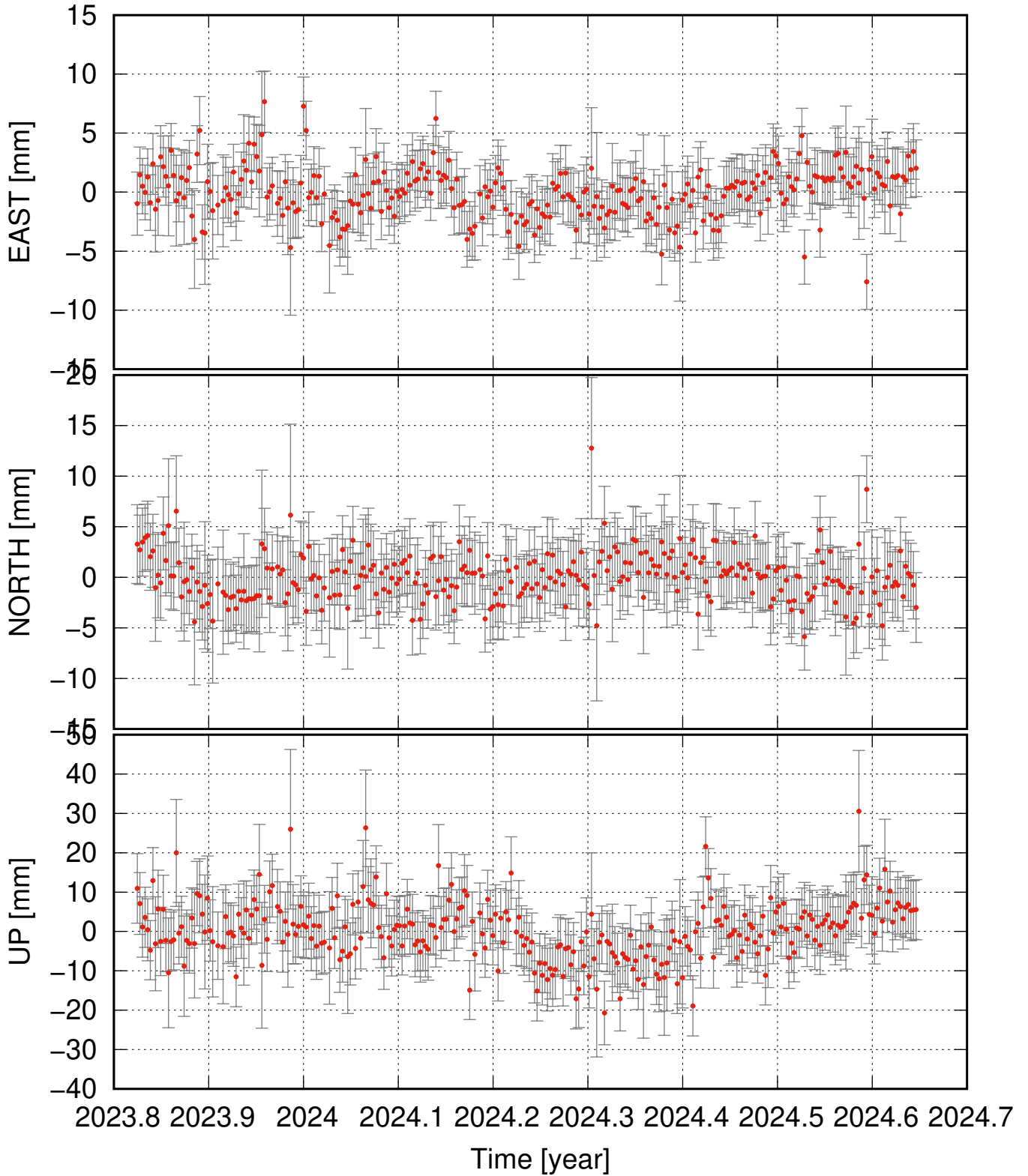
VOFJ residual time series (some major events removed as well)
