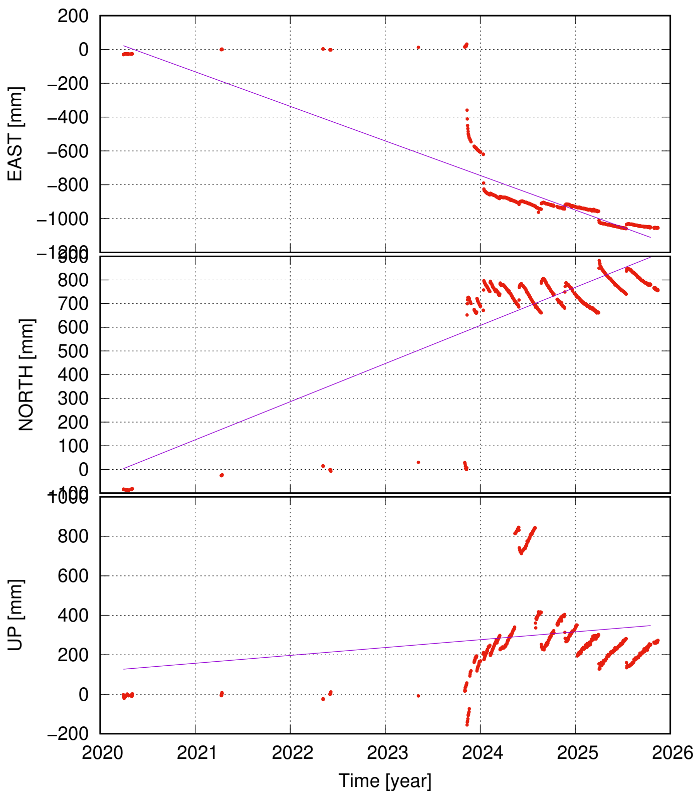
VMOS ( , ) time series (IGb20) ve = +- ; vn = +- ; vu = +- mm/yr
