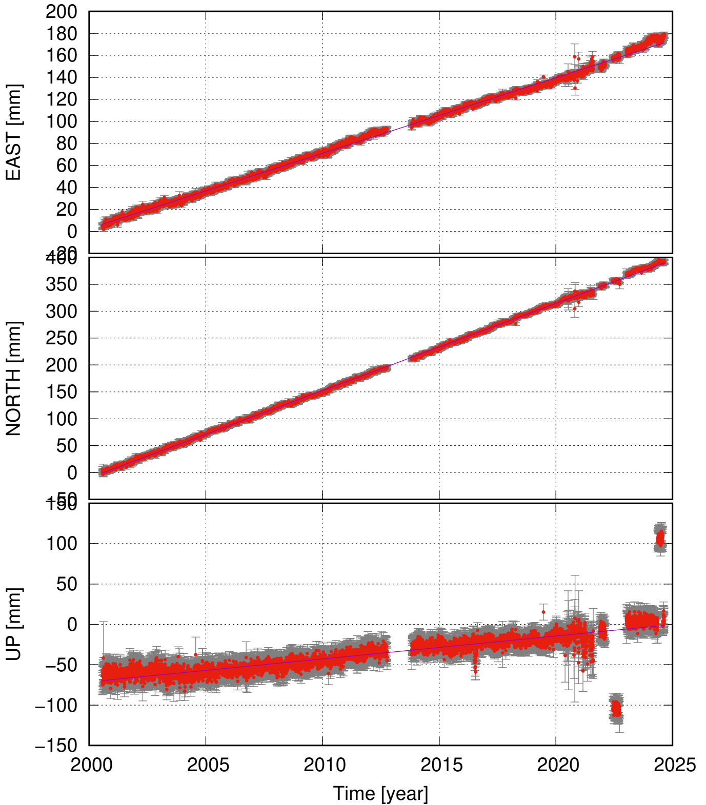
VMEY (63.43, -20.29) time series (ITRF 2014) v_e = 6.85 \pm 0.10 ; v_n = 16.23 \pm 0.10 ; v_u = 2.84 \pm 0.70 mm/yr
