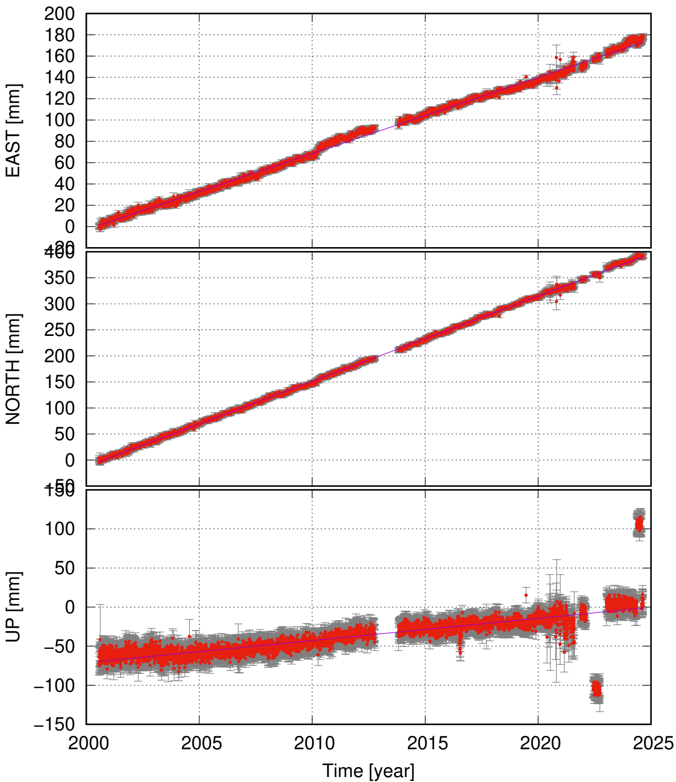
VMEY (63.43, -20.29) time series (ITRF 2014) v_e = 7.13 \pm 0.11 ; v_n = 16.35 \pm 0.10 ; v_u = 2.84 \pm 0.70 mm/yr
