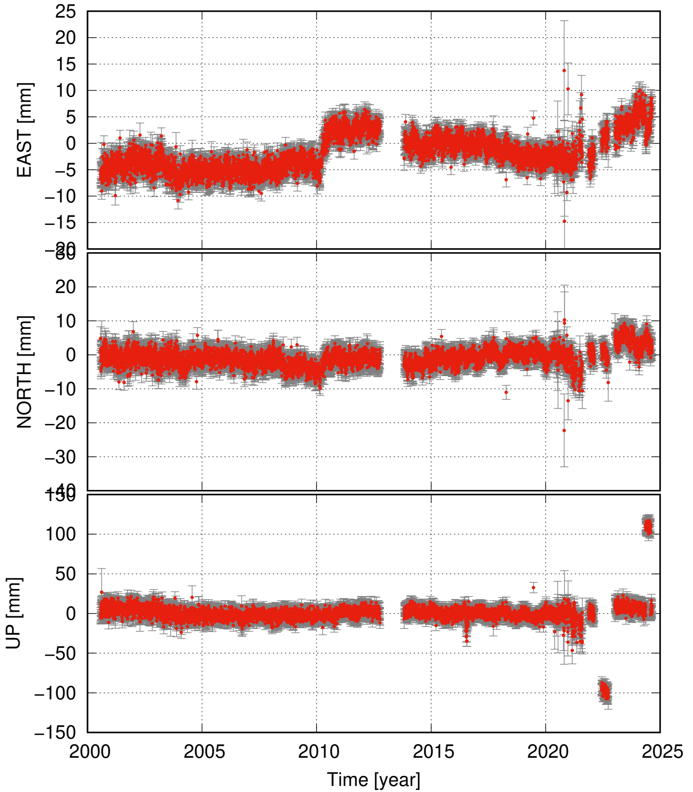
VMEY detrended and seasonal signal removed
