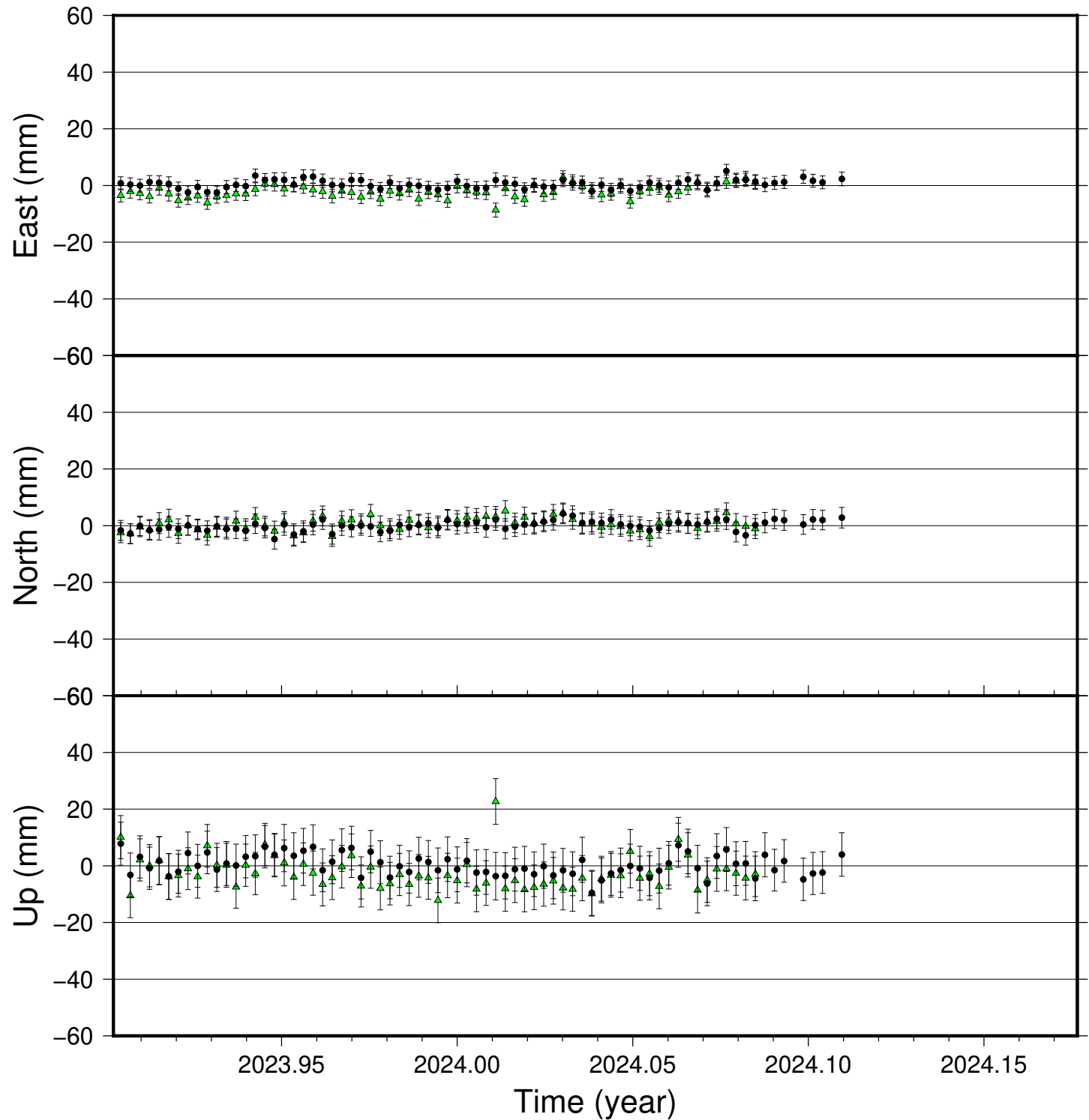
VMEY time series (IGS 2014), last 100 days
