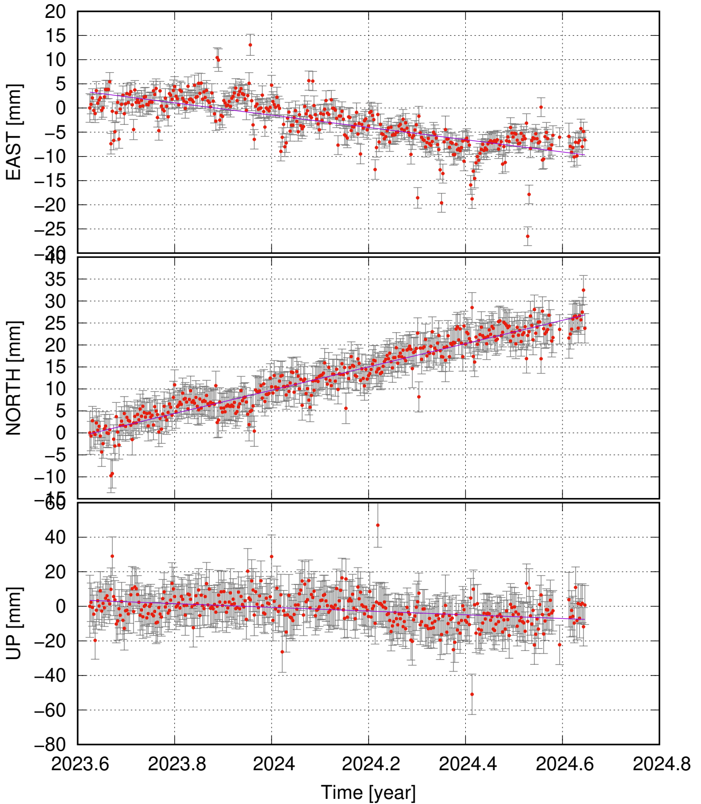
VARG (66.03, -17.68) time series (ITRF 2014) v_e = -12.69 \pm 3.29 ; v_n = 26.50 \pm 2.34 ; v_u = -10.73 \pm 7.94 mm/yr
