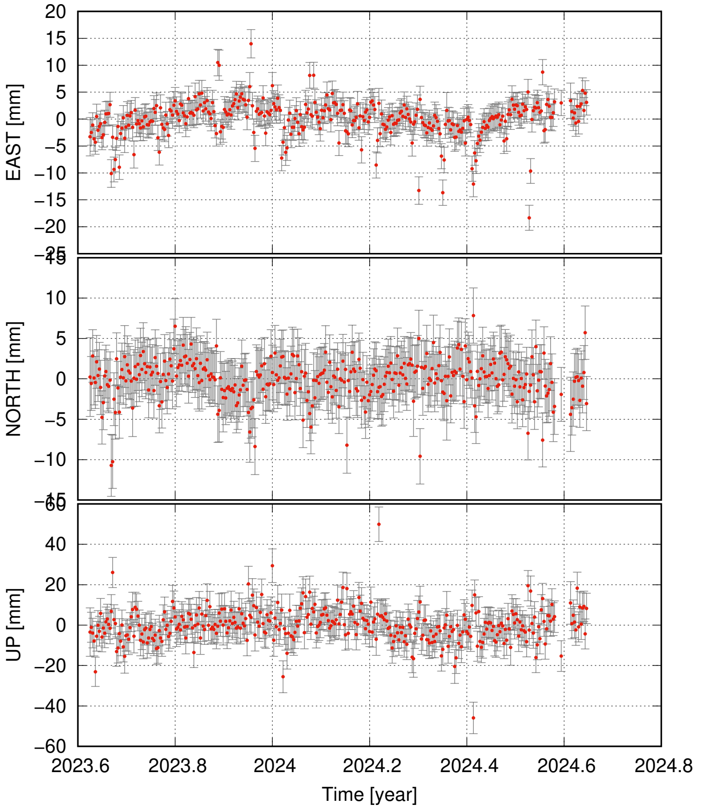
VARG residual time series (some major events removed as well)
