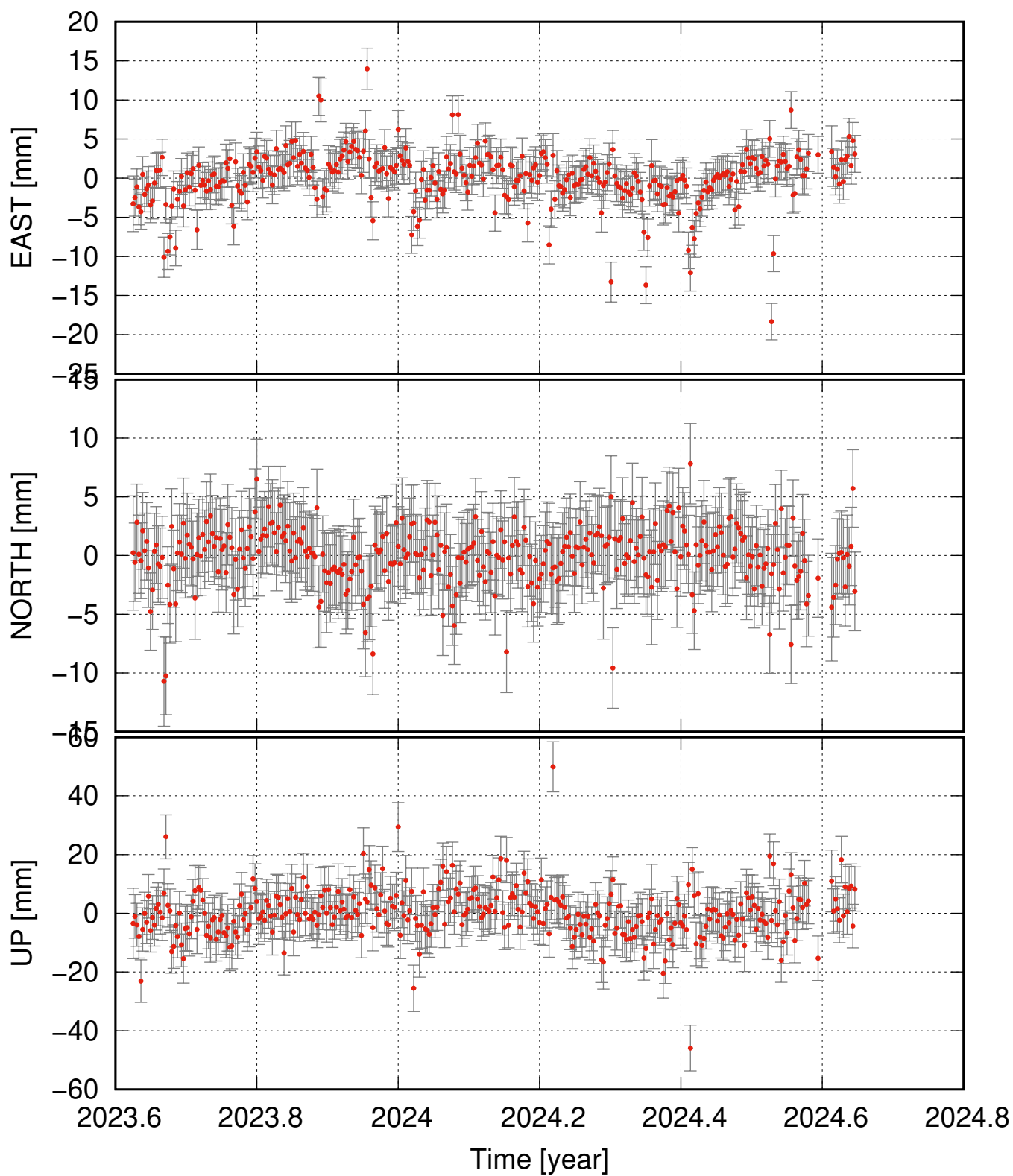
VARG residual time series
