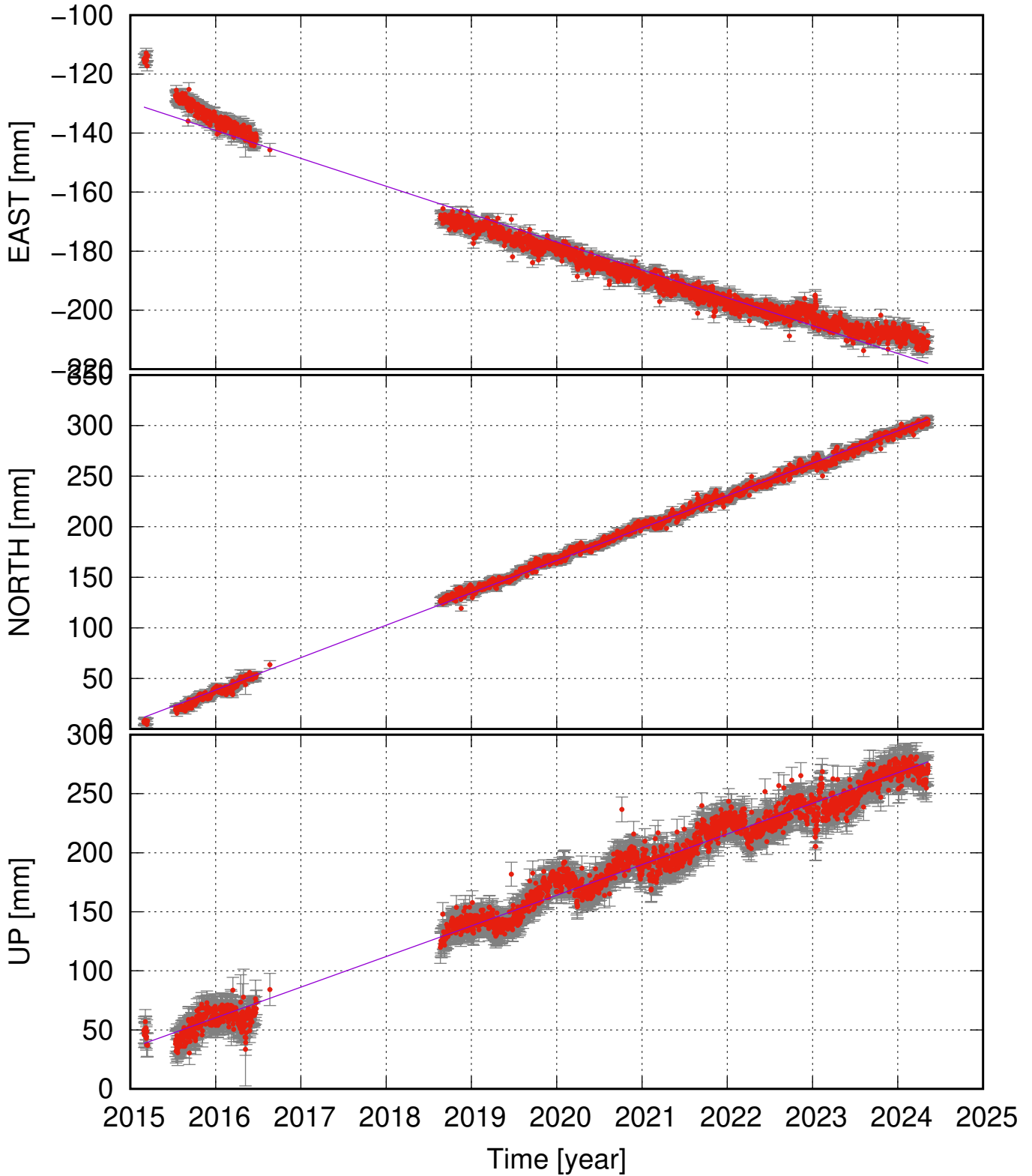
URHC (64.82, -17.15) time series (ITRF 2014) v_e = -9.44 \pm 0.45 ; v_n = 32.02 \pm 0.35 ; v_u = 25.94 \pm 0.96 mm/yr
