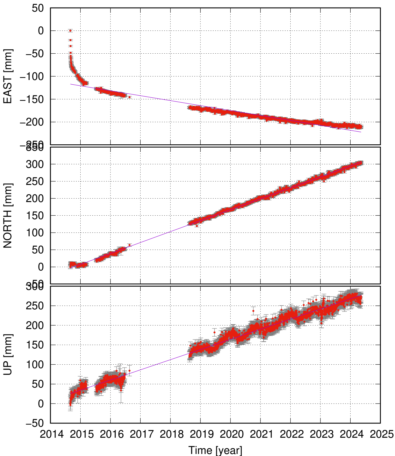
URHC (64.82, -17.15) time series (ITRF 2014) v_e = -10.83 \pm 0.91 ; v_n = 31.91 \pm 0.37 ; v_u = 25.93 \pm 0.91 mm/yr
