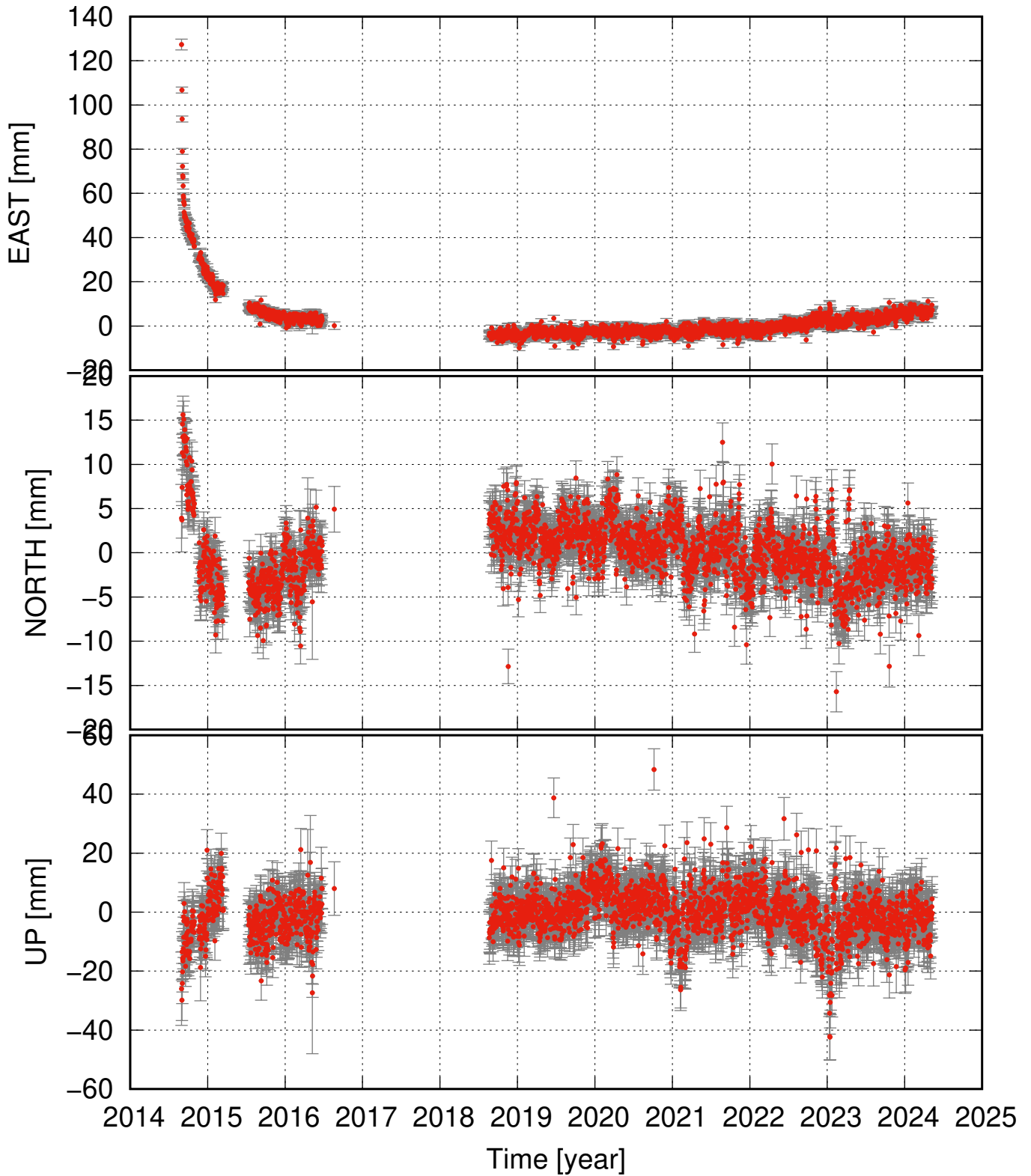
URHC detrended and seasonal signal removed
