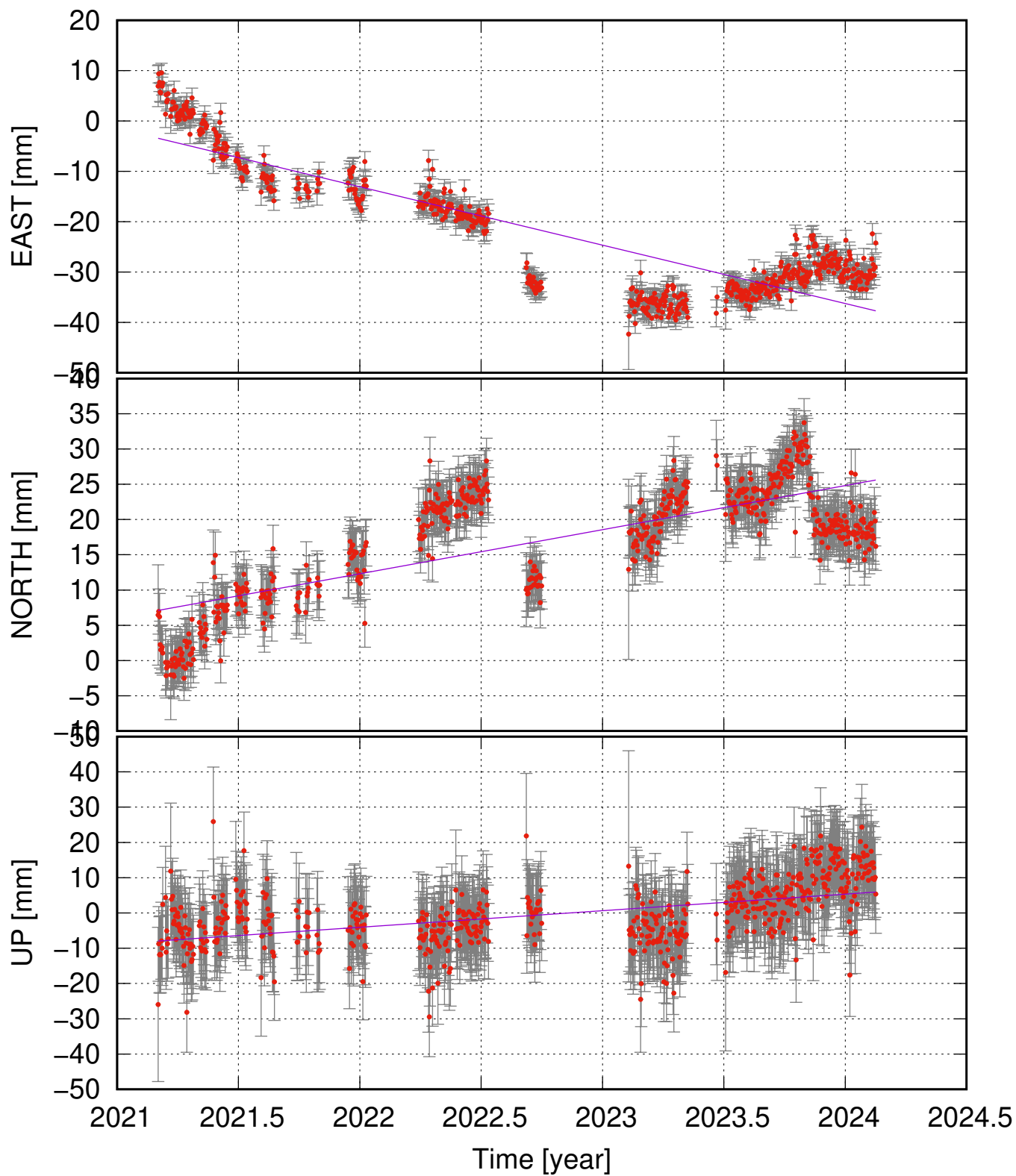
UNDH (63.97, -21.96) time series (ITRF 2014) v_e = -11.58 \pm 2.04 ; v_n = 6.26 \pm 1.79 ; v_u = 4.70 \pm 2.52 mm/yr
