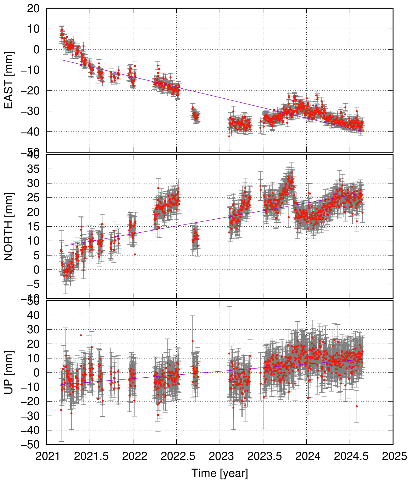
UNDH (63.97, -21.96) time series (ITRF 2014) v_e = -10.03 \pm 1.65 ; v_n = 5.33 \pm 1.42 ; v_u = 5.02 \pm 2.07 mm/yr
