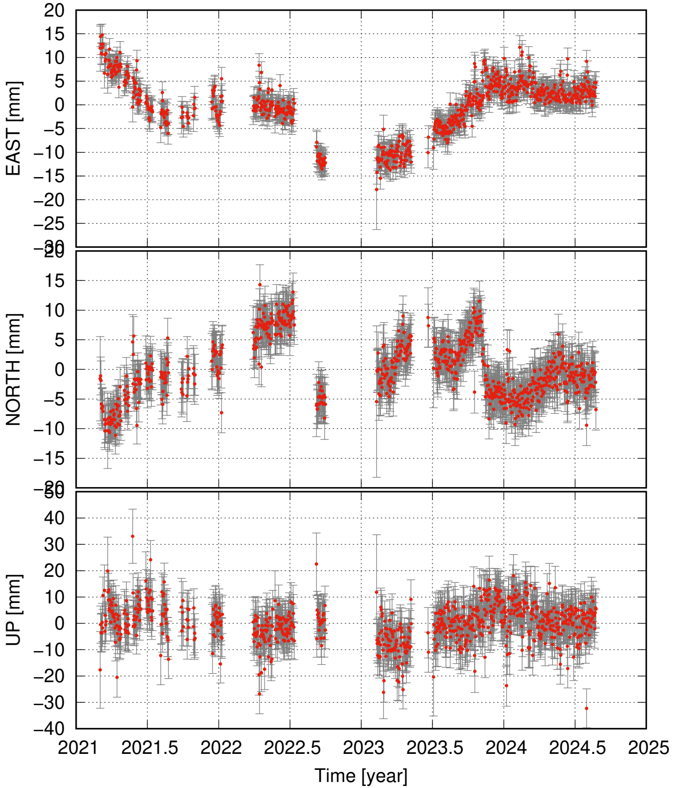
UNDH residual time series
