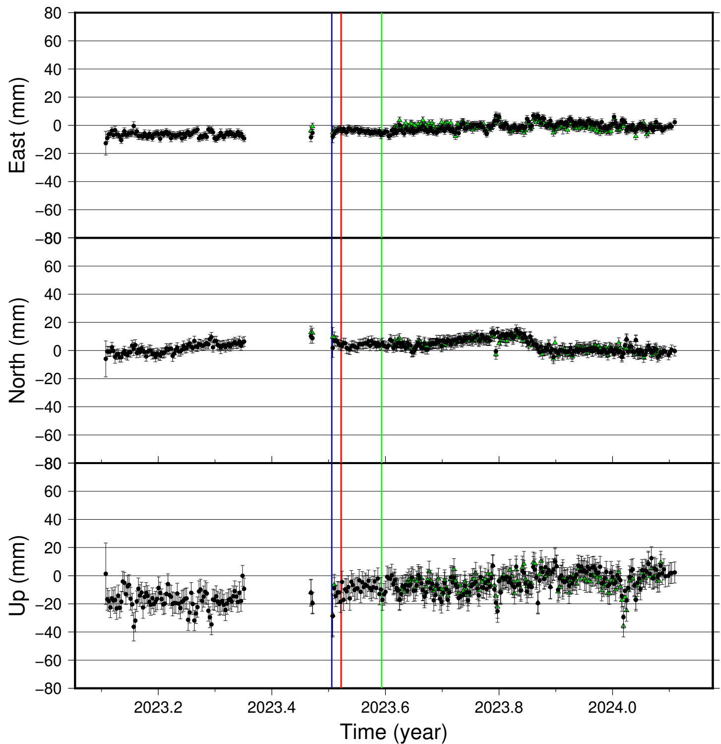
UNDH time series (IGS 2014), last 400 days
