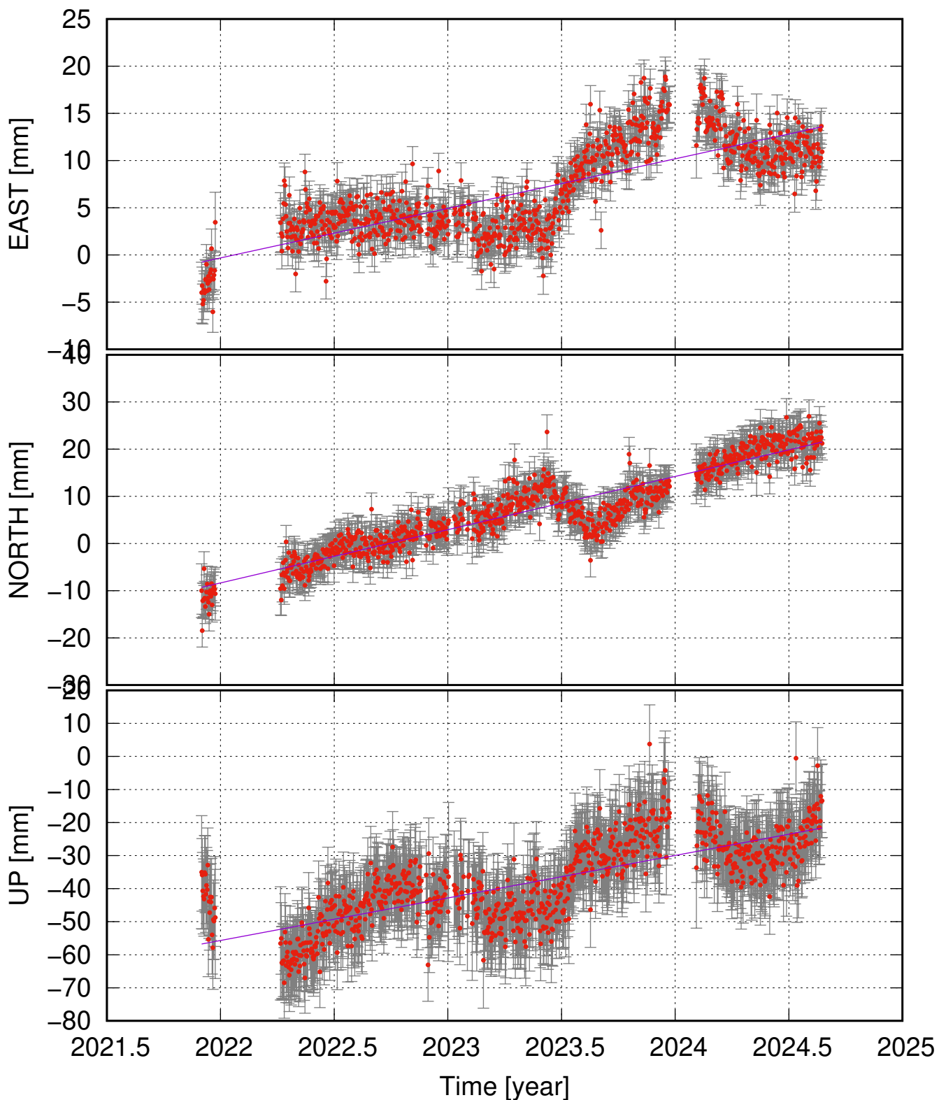
TORK (63.91, -19.07) time series (ITRF 2014) v_e = 5.25 \pm 1.14 ; v_n = 11.28 \pm 1.17 ; v_u = 12.86 \pm 3.04 mm/yr
