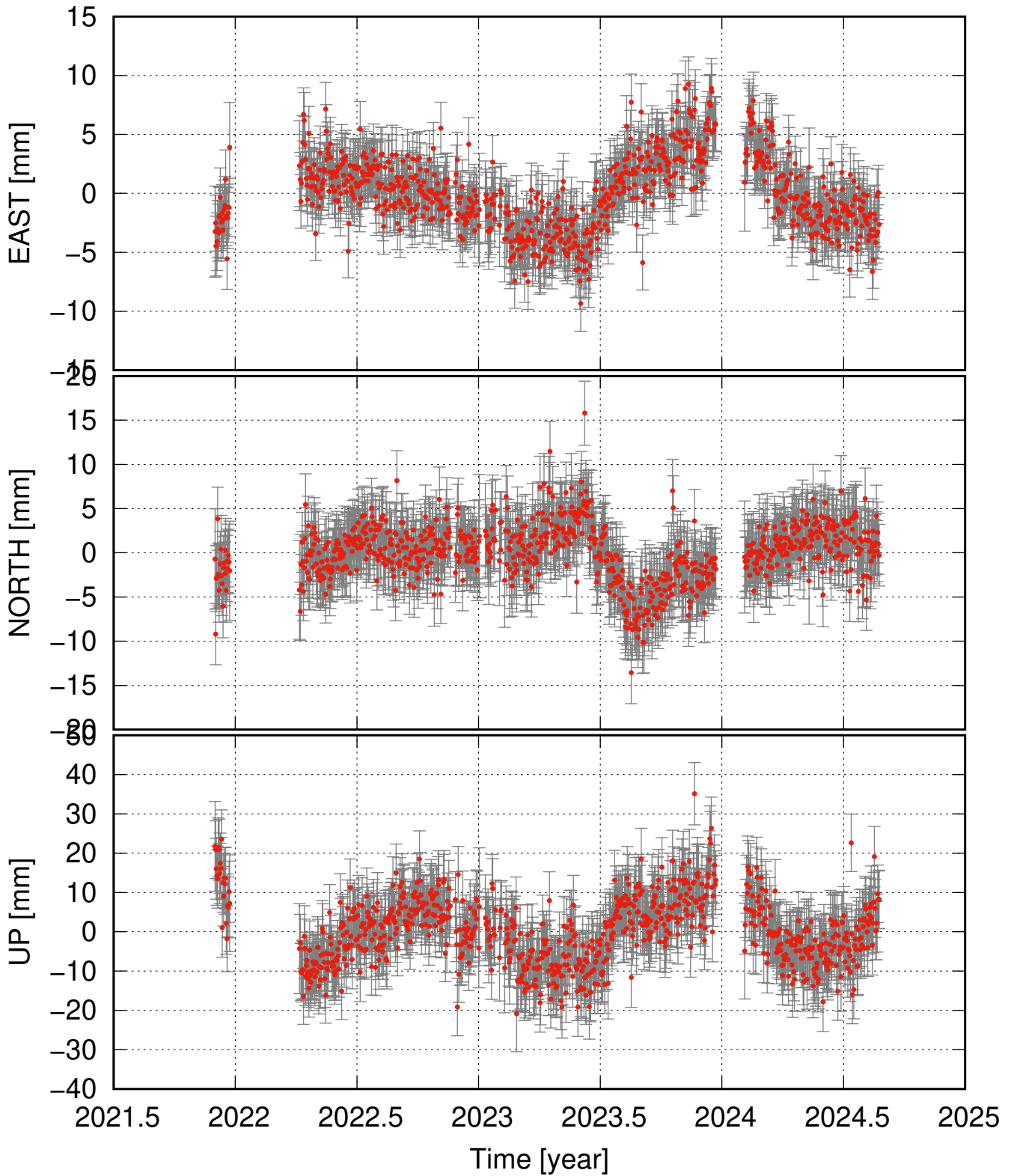
TORK residual time series (some major events removed as well)
