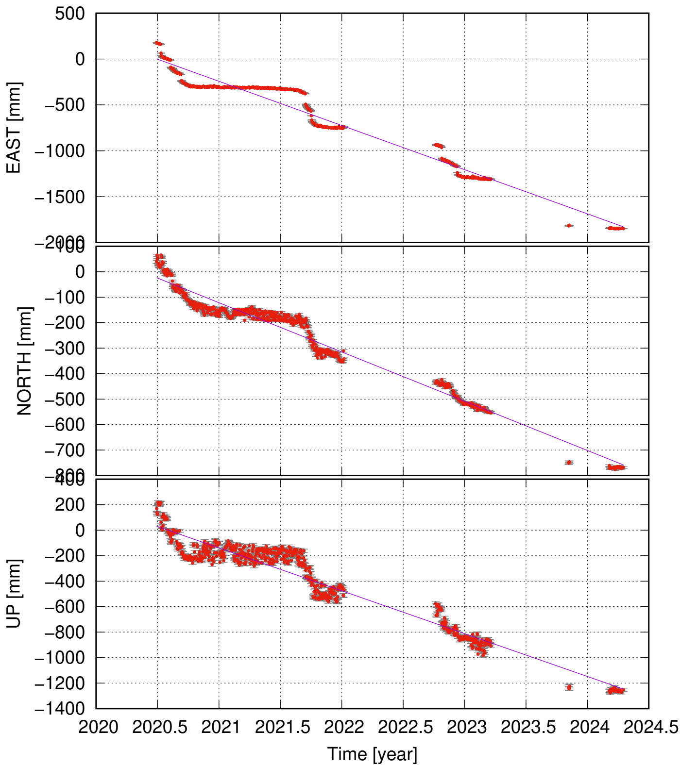
TKJ2 (63.65, -19.35) time series (ITRF 2014) v_e = -481.70 \pm 27.49 ; v_n = -193.34 \pm 8.90 ; v_u = -336.29 \pm 23.36 mm/yr
