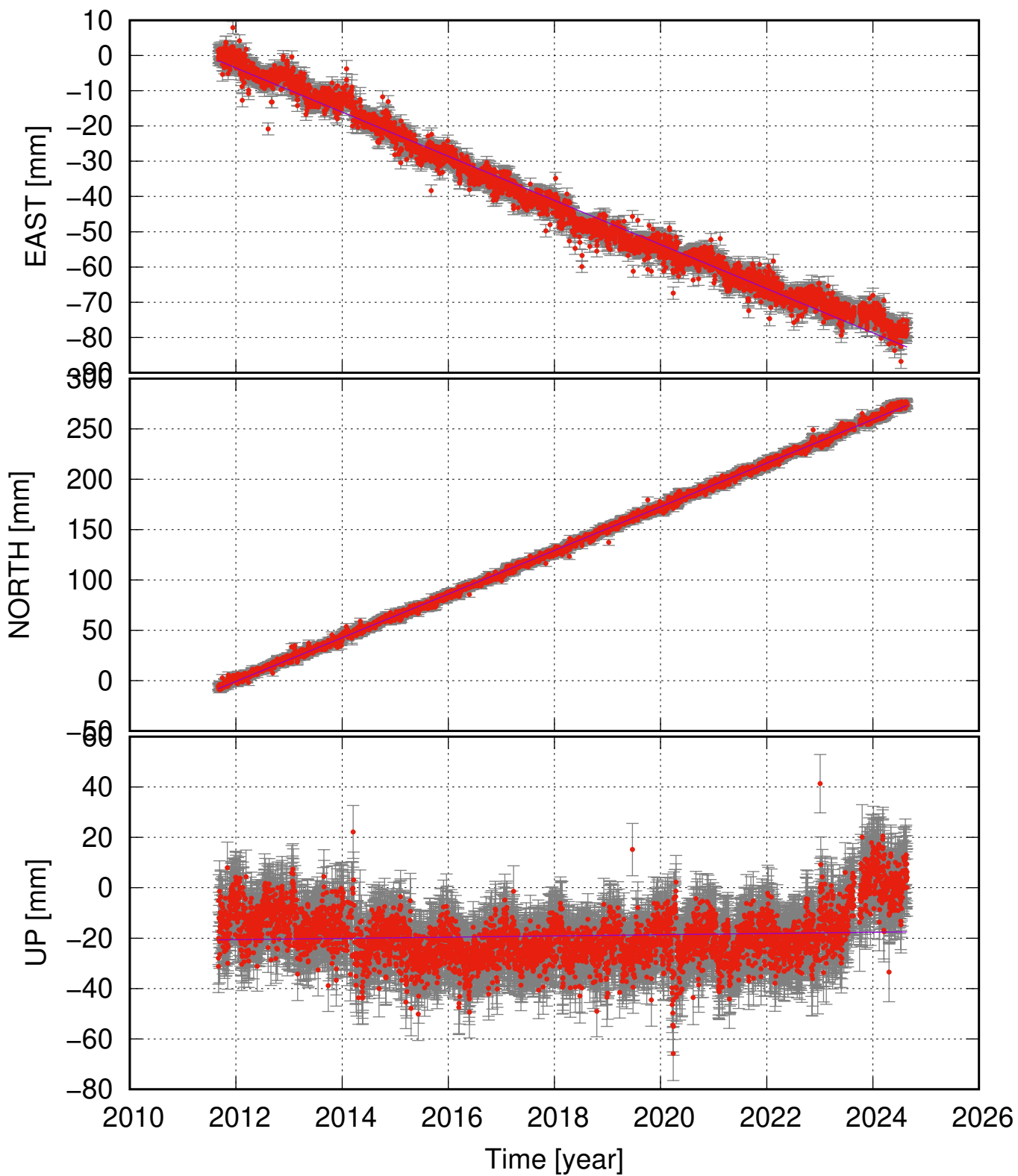
THRC (65.90, -17.01) time series (ITRF 2014) v_e = -6.26 \pm 0.22 ; v_n = 21.67 \pm 0.18 ; v_u = 0.24 \pm 0.77 mm/yr
