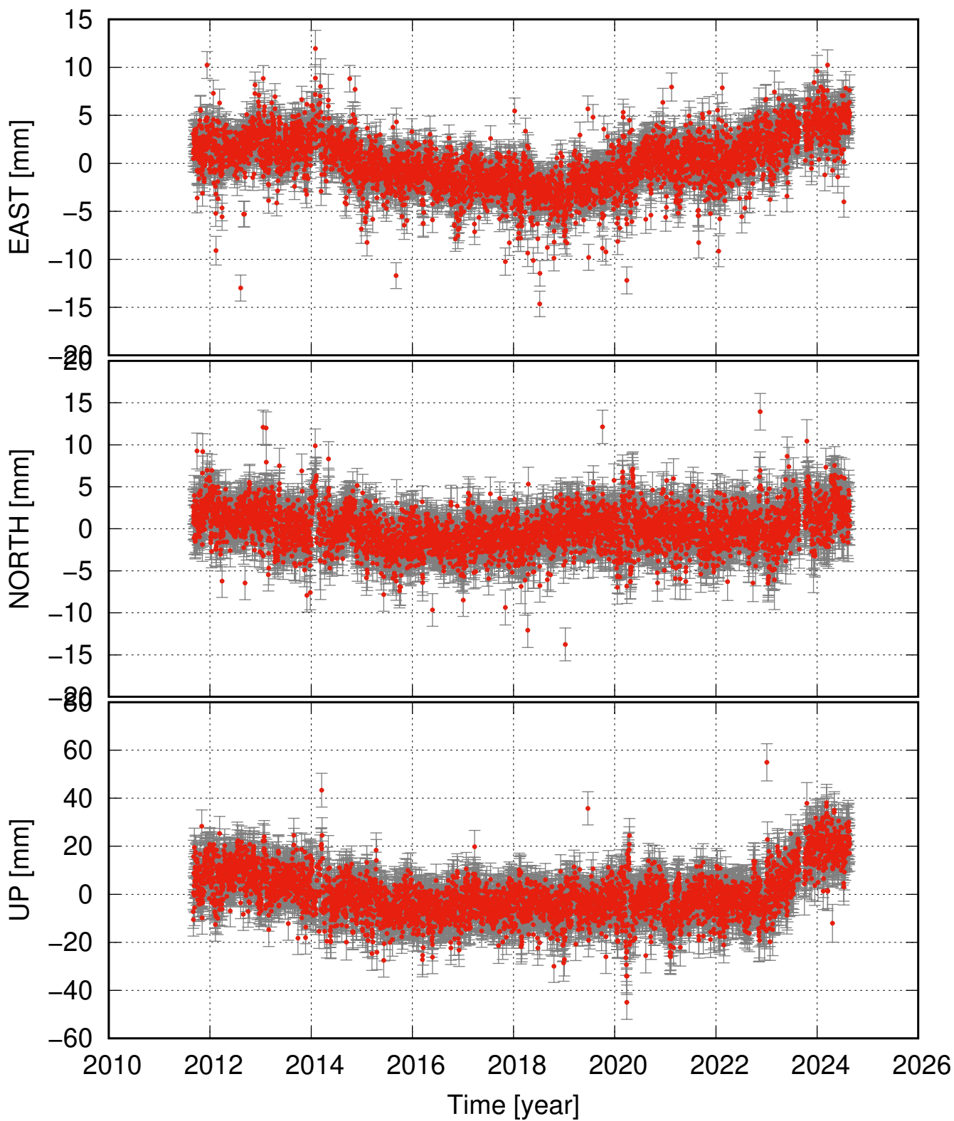
THRC detrended and seasonal signal removed
