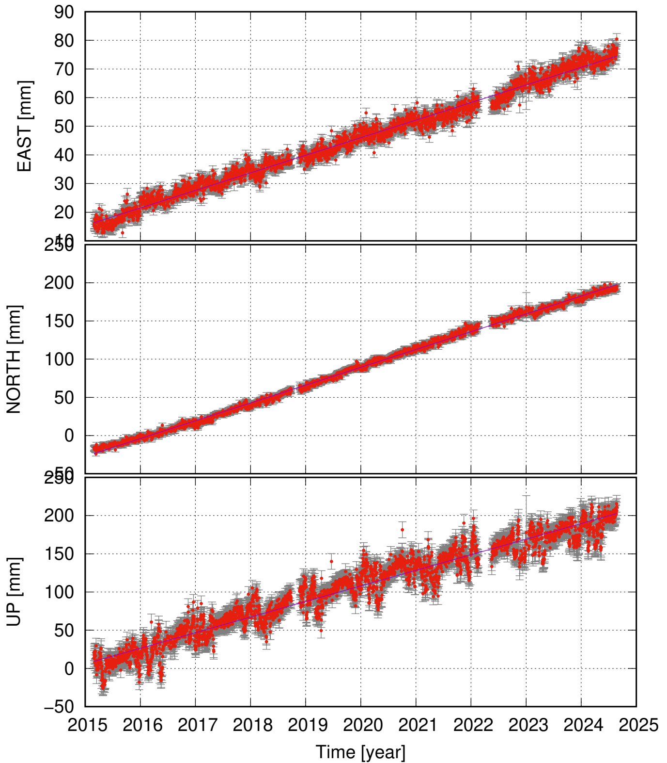
THOC (64.93, -16.68) time series (ITRF 2014) v_e = 6.13 \pm 0.21 ; v_n = 23.31 \pm 0.33 ; v_u = 20.41 \pm 1.44 mm/yr
