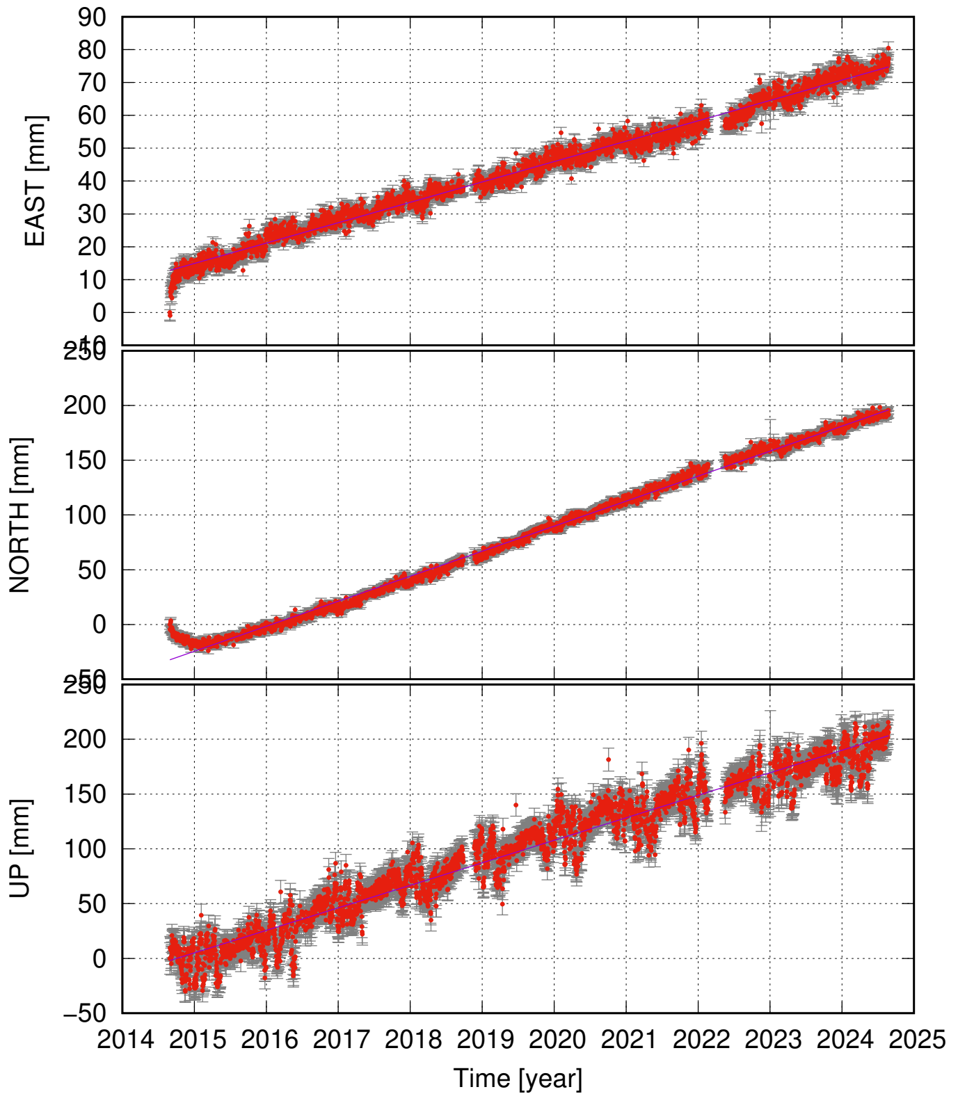
THOC (64.93, -16.68) time series (ITRF 2014) v_e = 6.20 \pm 0.21 ; v_n = 22.84 \pm 0.48 ; v_u = 20.56 \pm 1.38 mm/yr
