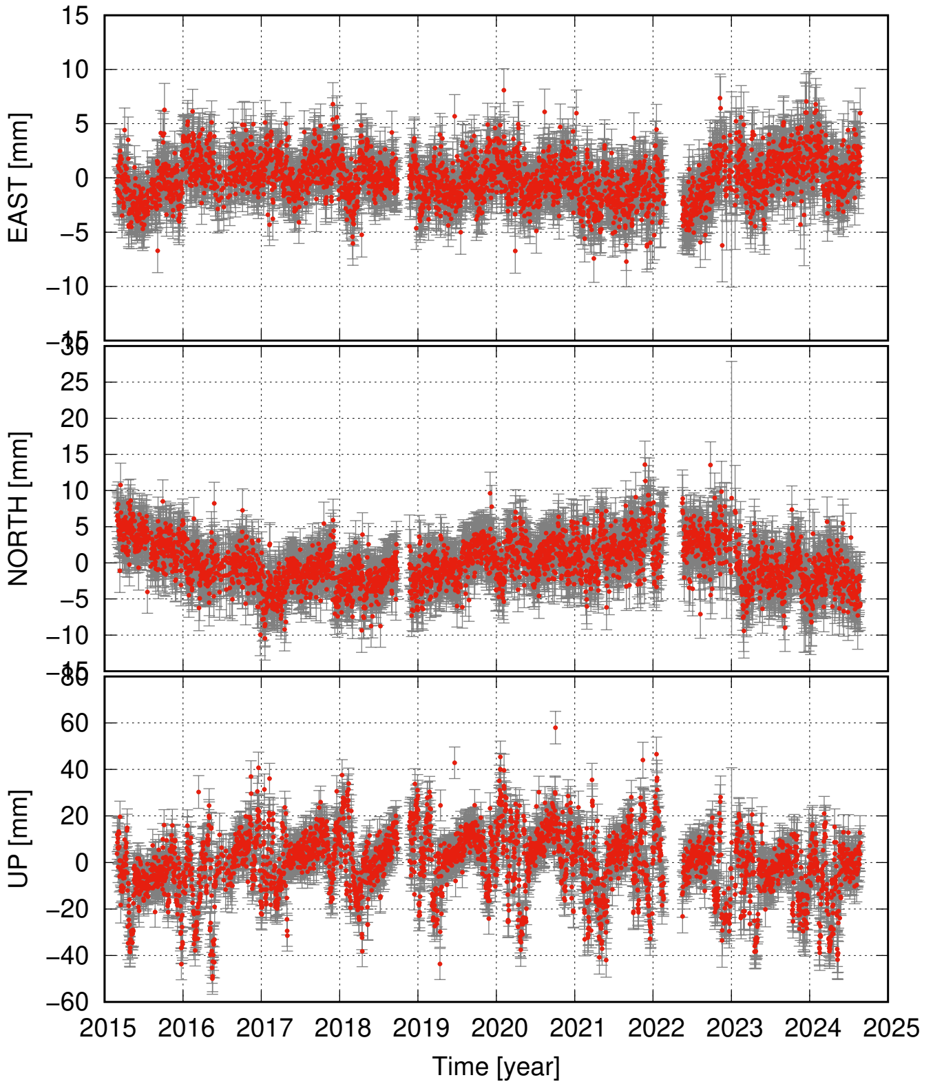
THOC residual time series (some major events removed as well)
