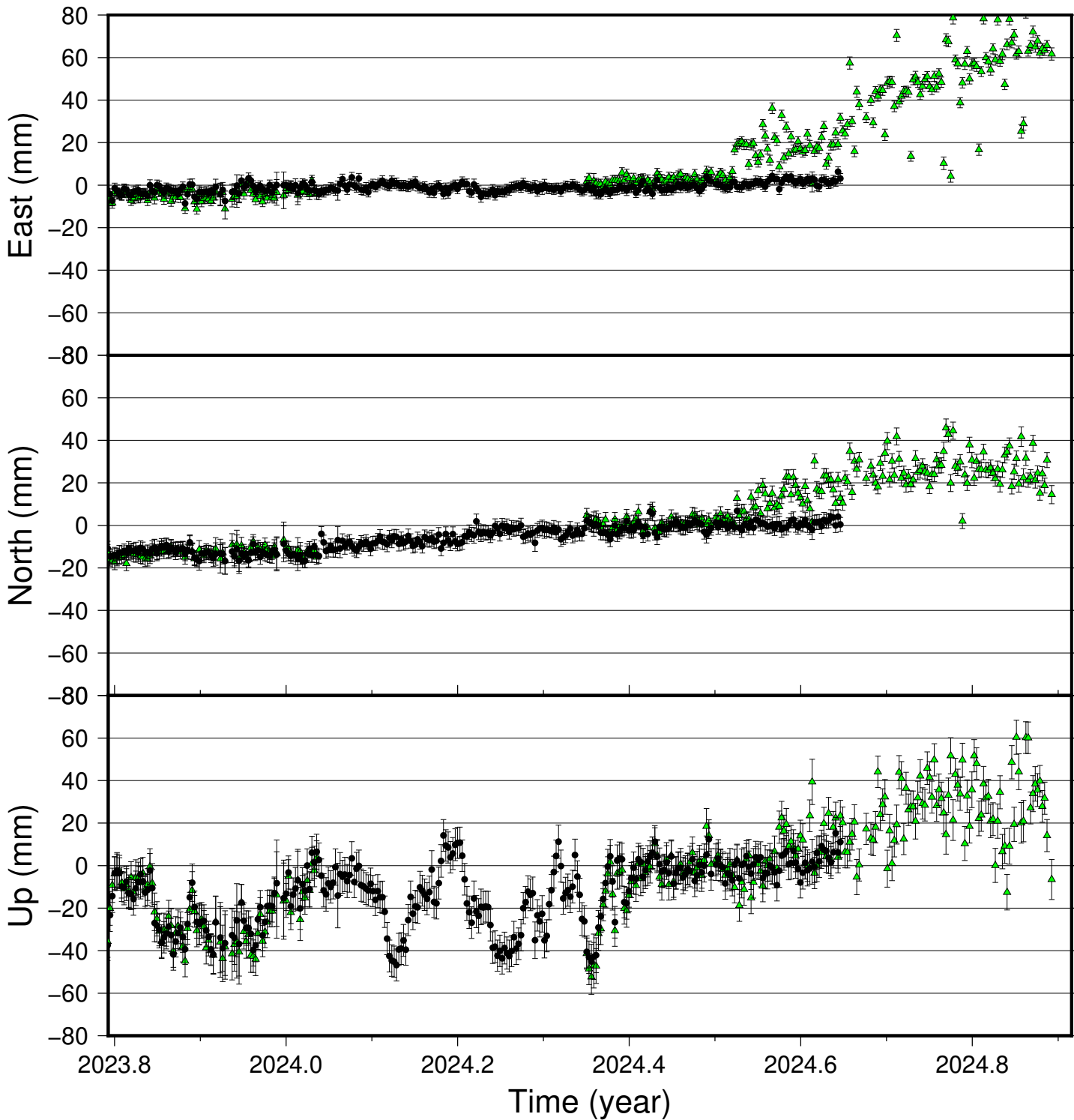
THOC time series (IGS 2014), last 400 days
