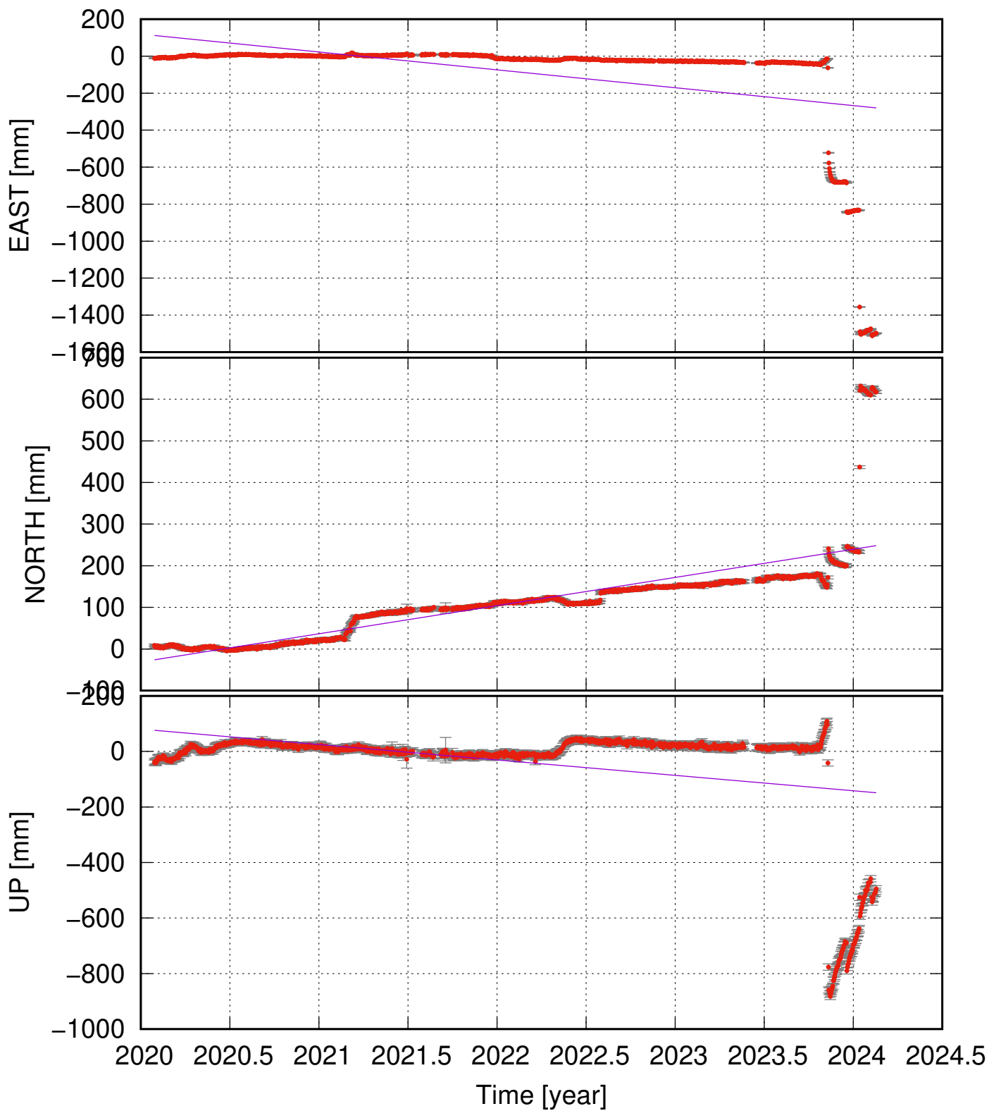
THOB (63.86, -22.44) time series (ITRF 2014) v_e = -96.66 \pm 58.35 ; v_n = 67.70 \pm 15.00 ; v_u = -55.50 \pm 40.07 mm/yr
