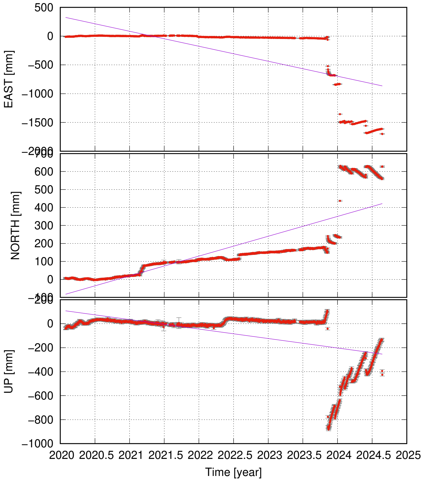
THOB (63.86, -22.44) time series (ITRF 2014) v_e = -260.56 \pm 88.86 ; v_n = 110.37 \pm 23.37 ; v_u = -78.97 \pm 35.87 mm/yr
