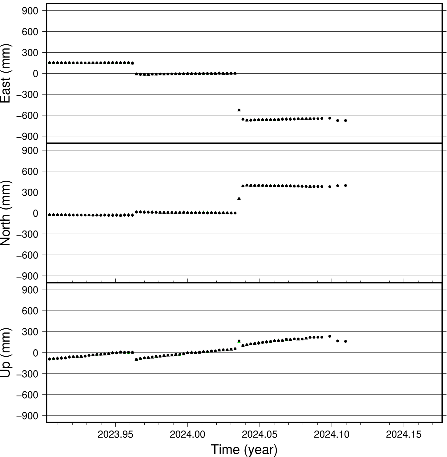
THOB time series (IGS 2014), last 100 days
