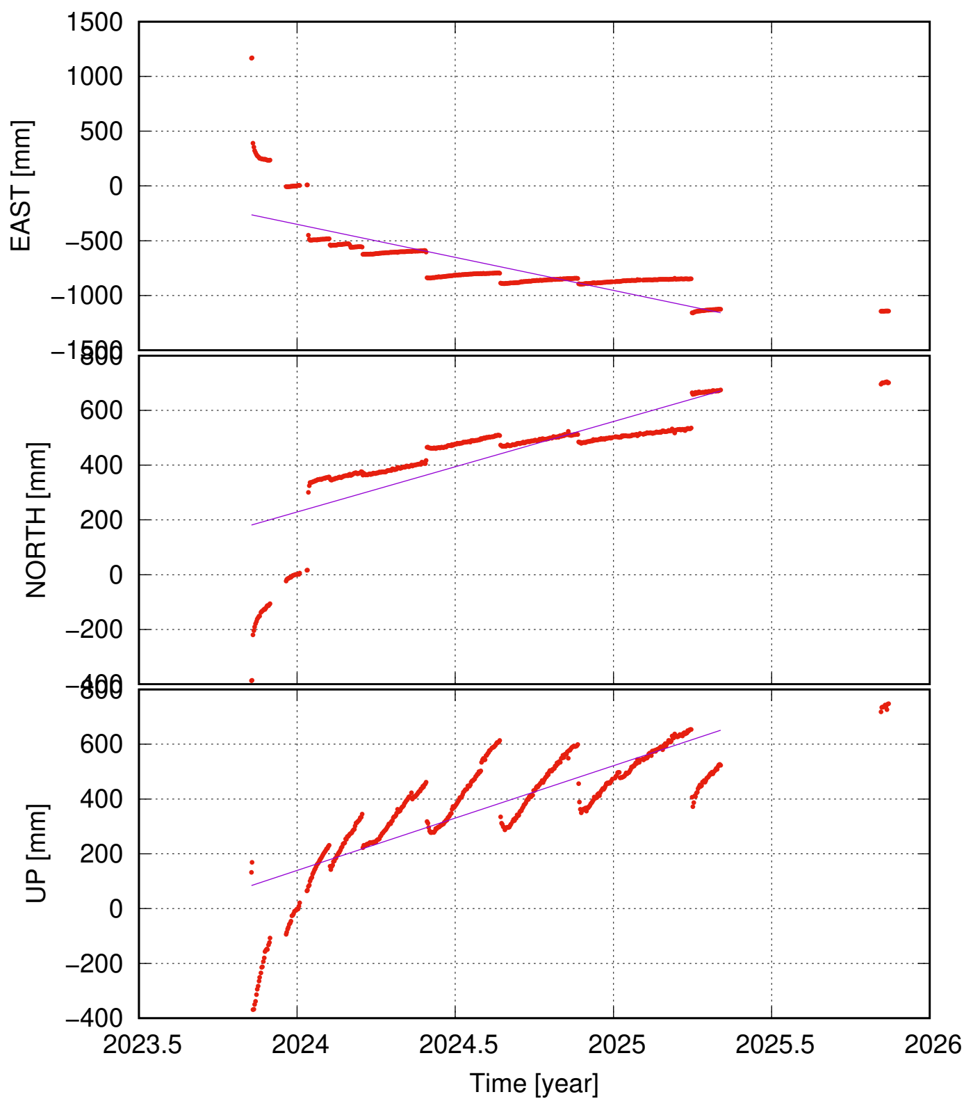
THNA ( , ) time series (IGb20) ve = +- ; vn = +- ; vu = +- mm/yr
