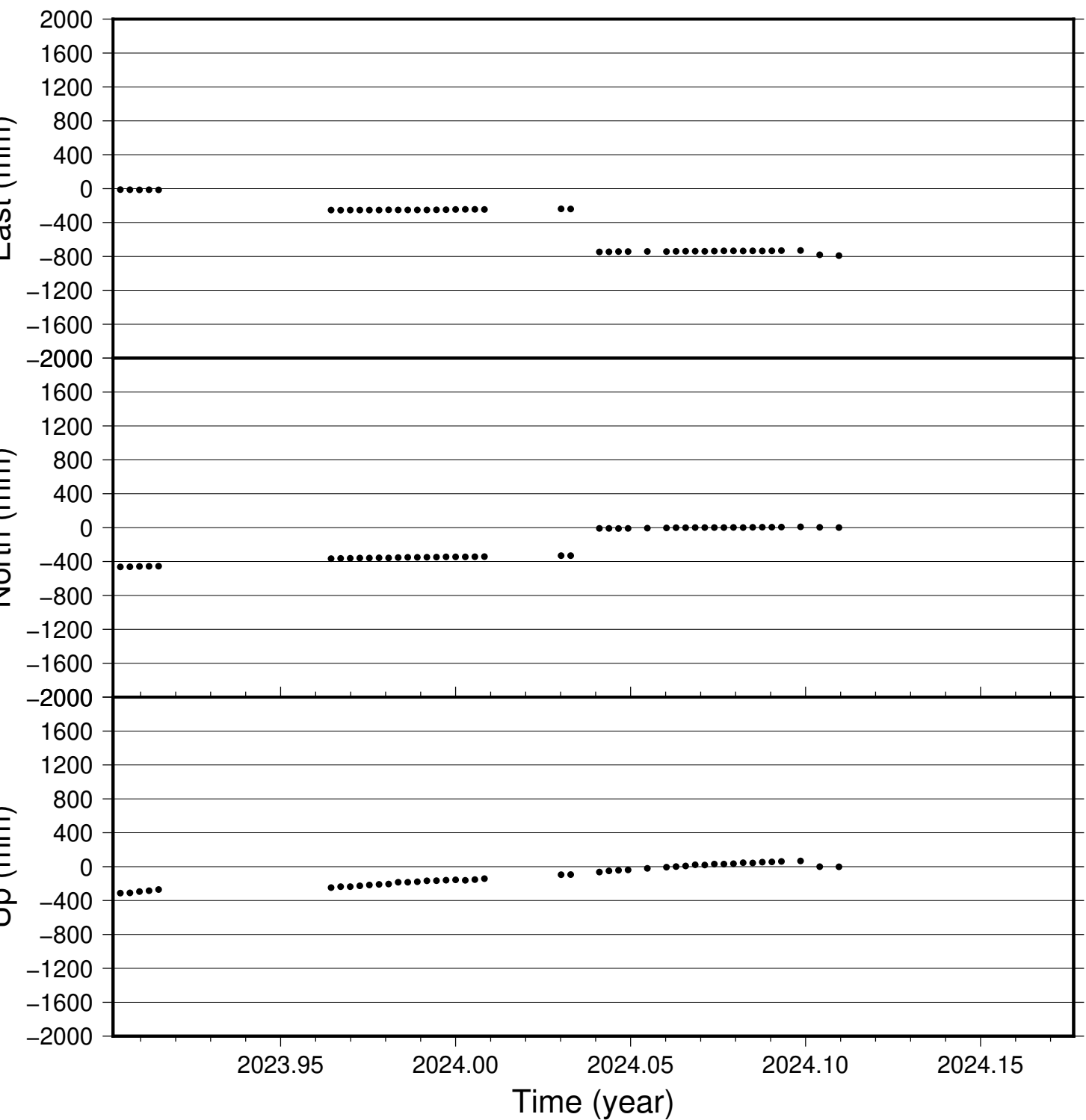
THNA time series (IGS 2014), last 100 days
