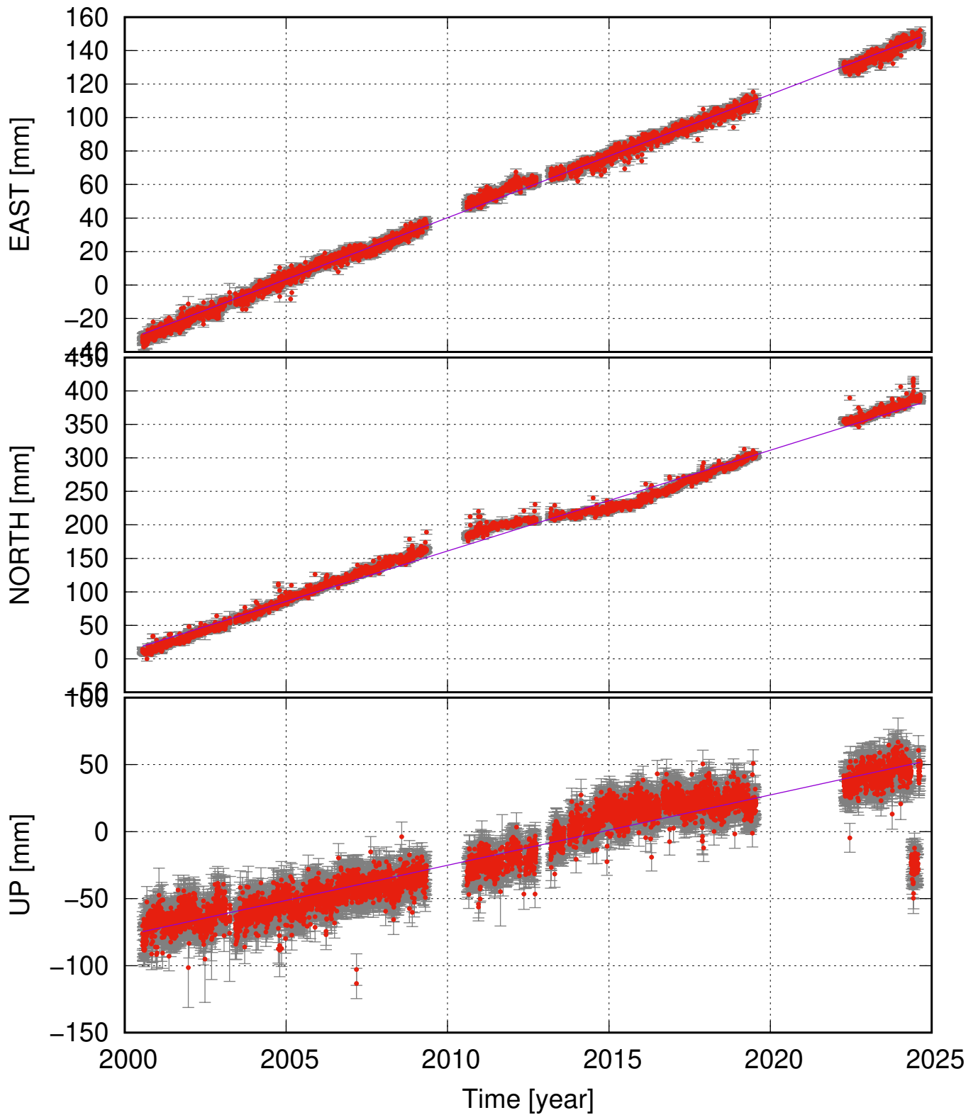
THEY (63.56, -19.64) time series (ITRF 2014) v_e = 7.36 \pm 0.10 ; v_n = 15.05 \pm 0.37 ; v_u = 5.24 \pm 0.51 mm/yr
