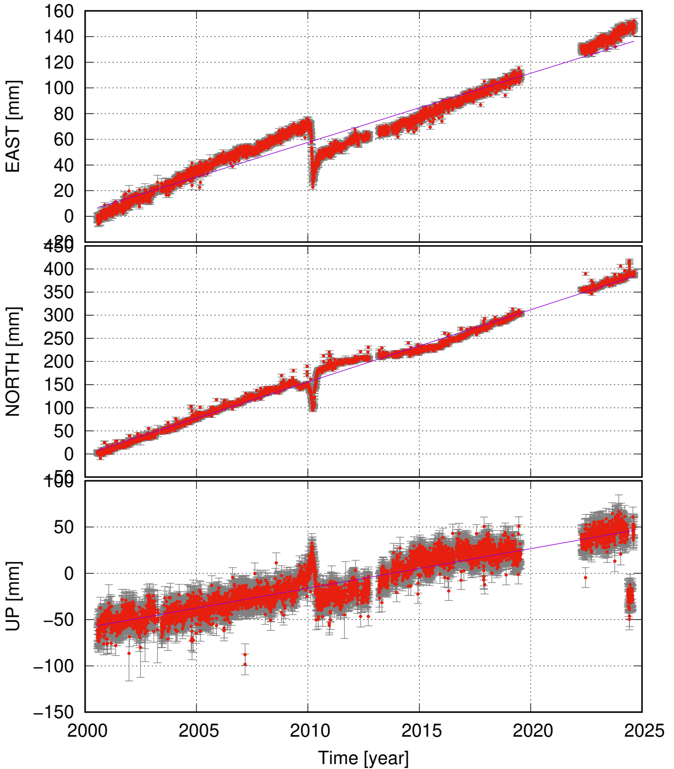
THEY (63.56, -19.64) time series (ITRF 2014) v_e = 5.38 \pm 0.34 ; v_n = 15.63 \pm 0.40 ; v_u = 4.28 \pm 0.50 mm/yr
