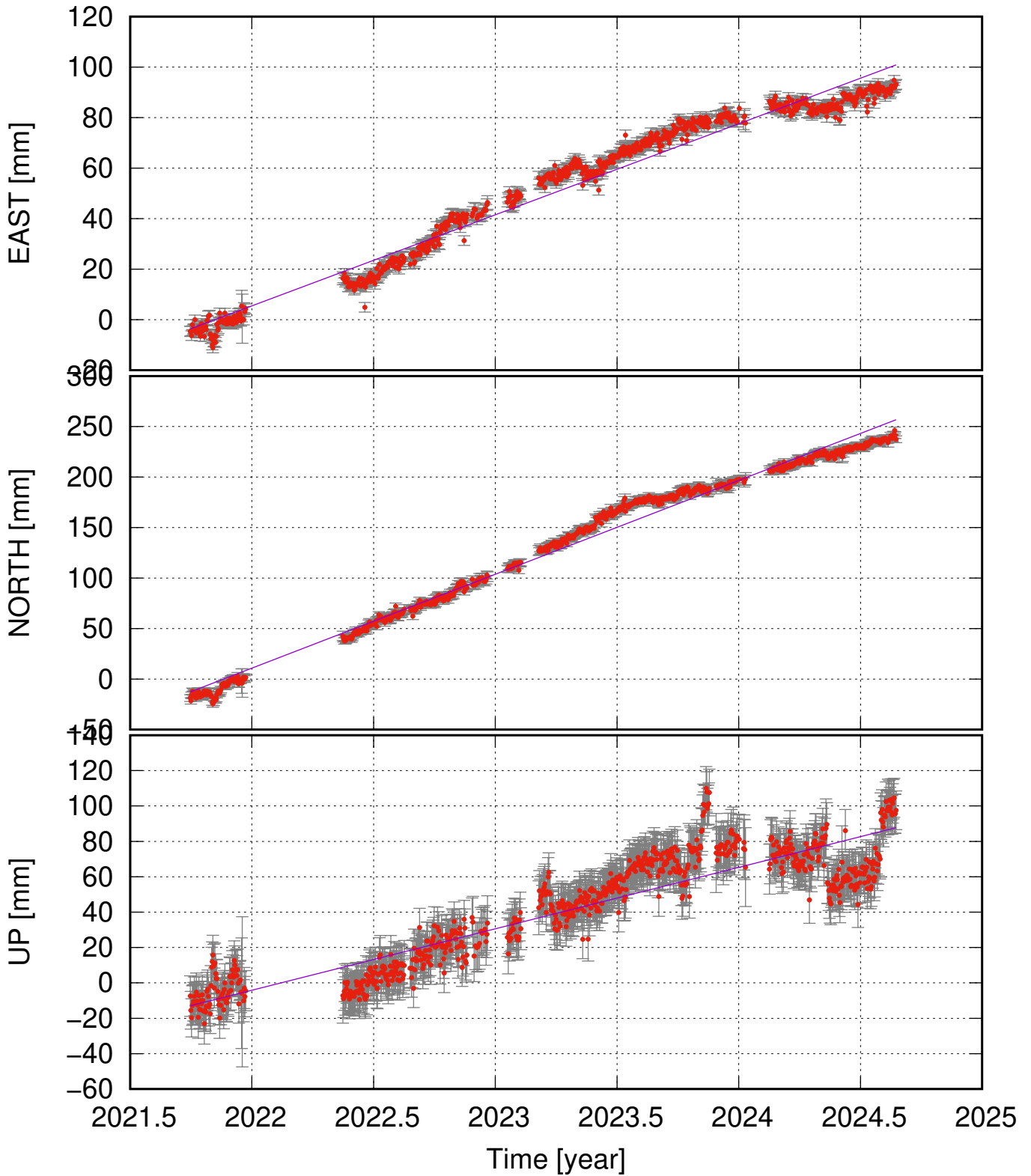
TANC (65.08, -16.74) time series (ITRF 2014) v_e = 36.05 \pm 1.92 ; v_n = 92.92 \pm 3.20 ; v_u = 34.74 \pm 4.54 mm/yr
