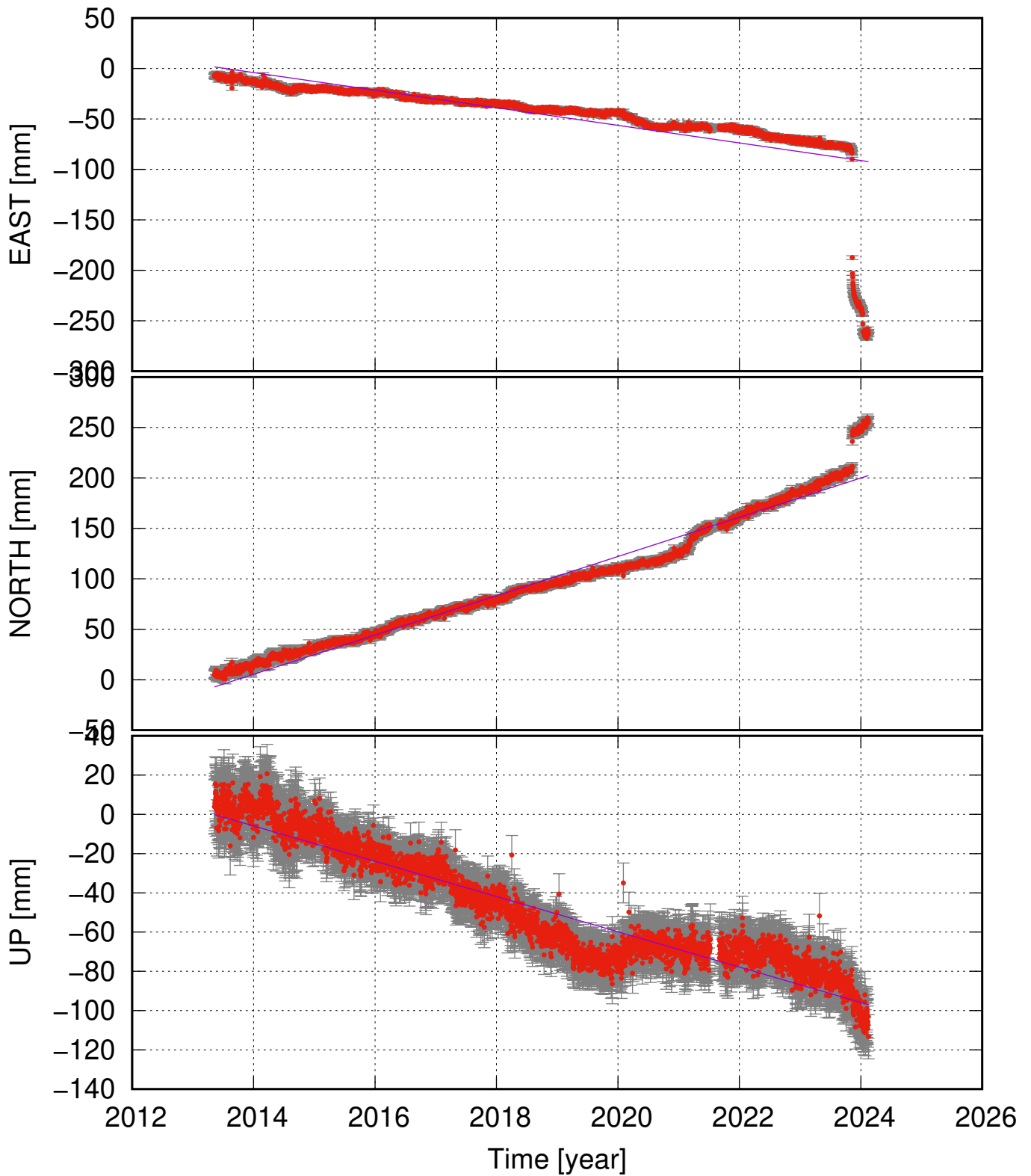
SYRF (63.84, -22.65) time series (ITRF 2014) v_e = -8.71 \pm 2.35 ; v_n = 19.44 \pm 1.03 ; v_u = -8.99 \pm 0.86 mm/yr
