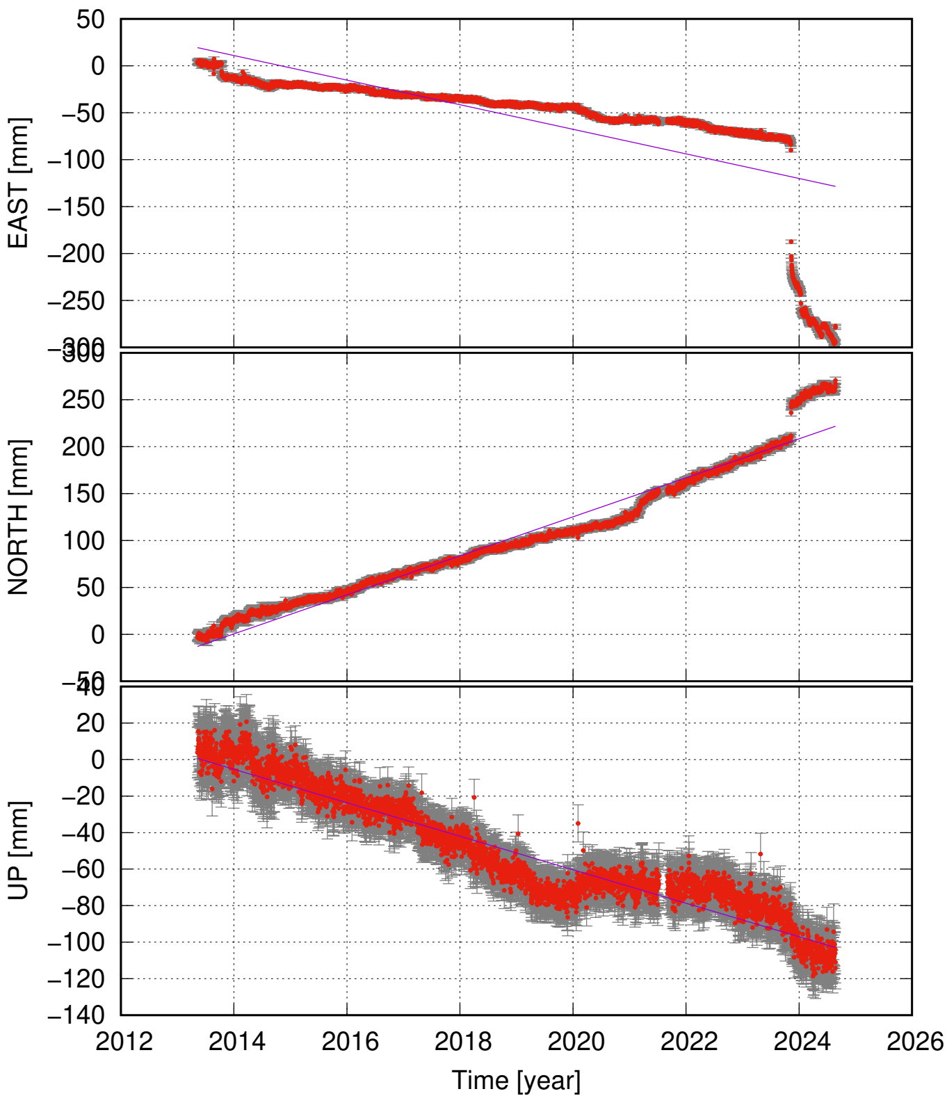
SYRF (63.84, -22.65) time series (ITRF 2014) ve = -13.09 \pm 3.89 ; vn = 20.76 \pm 1.32 ; vu = -9.17 \pm 0.82 mm/yr
