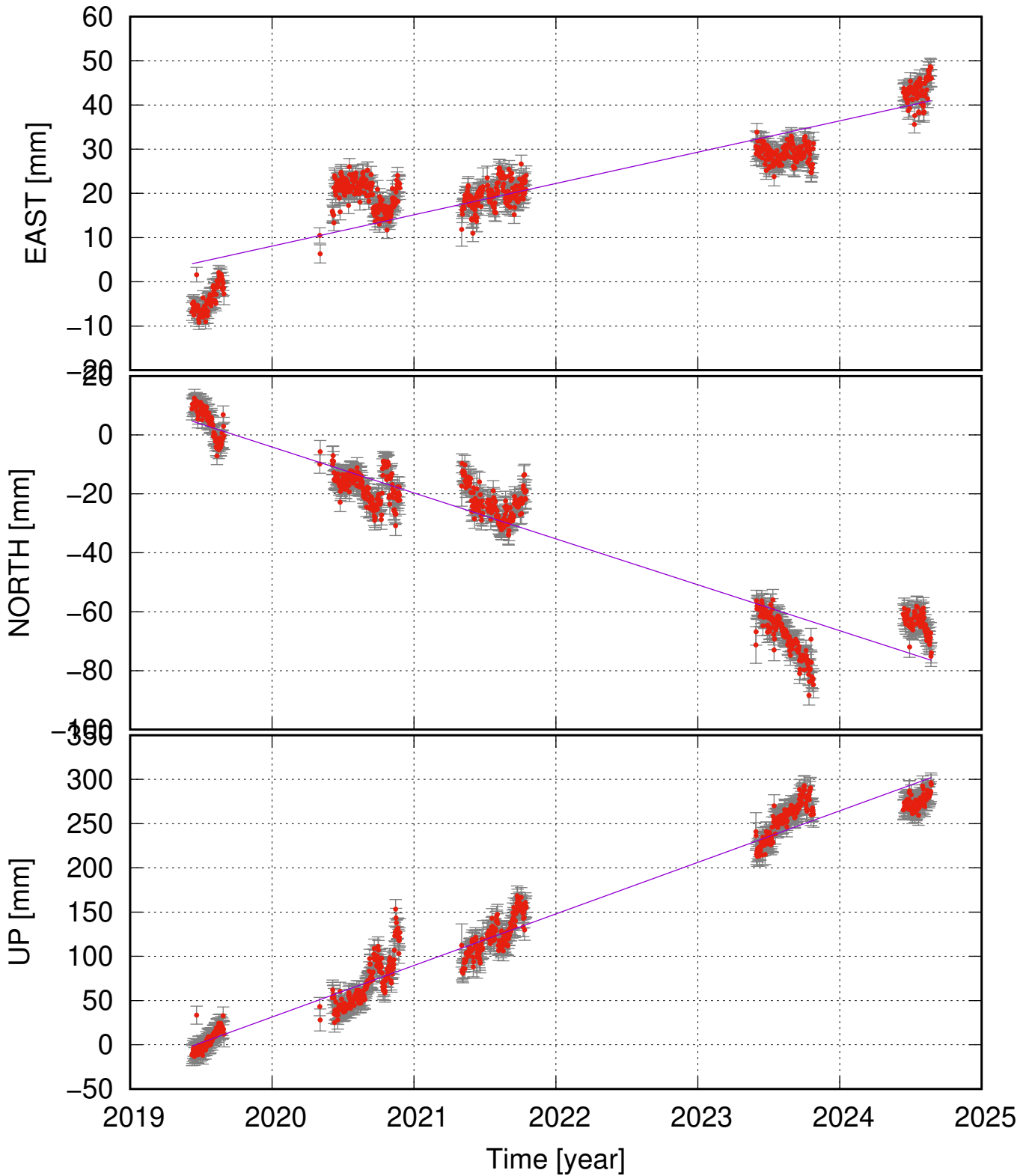
SVV2 (64.39, -17.32) time series (ITRF 2014) ve = 7.08 ± 1.18; vn = -15.58 ± 1.50; vu = 58.28 ± 3.38 mm/yr
