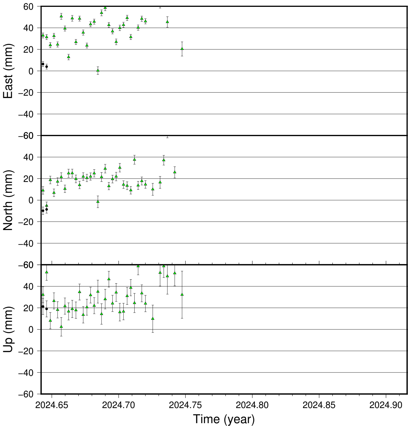
SVV2 time series (IGS 2014), last 100 days
