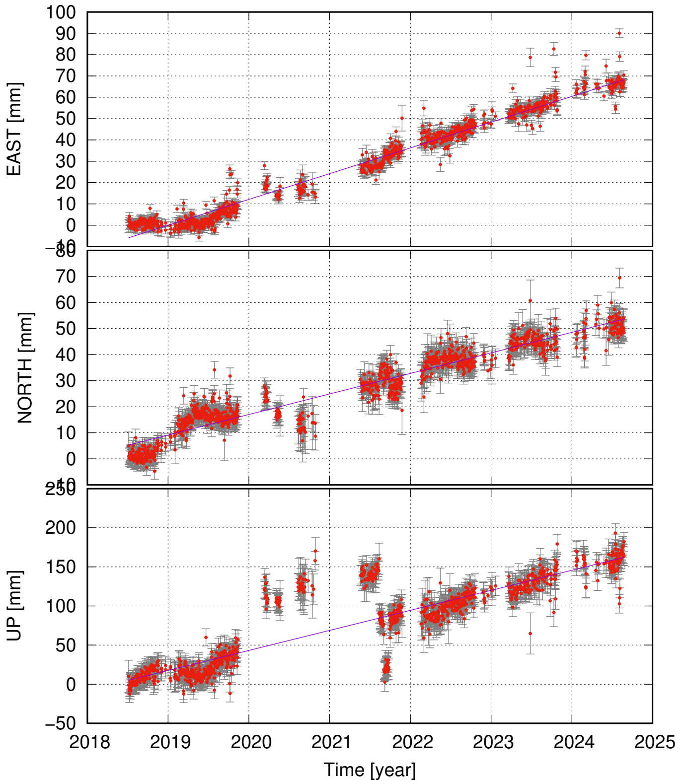
SVIN (64.01, -16.82) time series (ITRF 2014) v_e = 12.07 \pm 0.64 ; v_n = 7.88 \pm 0.72 ; v_u = 25.59 \pm 4.09 mm/yr
