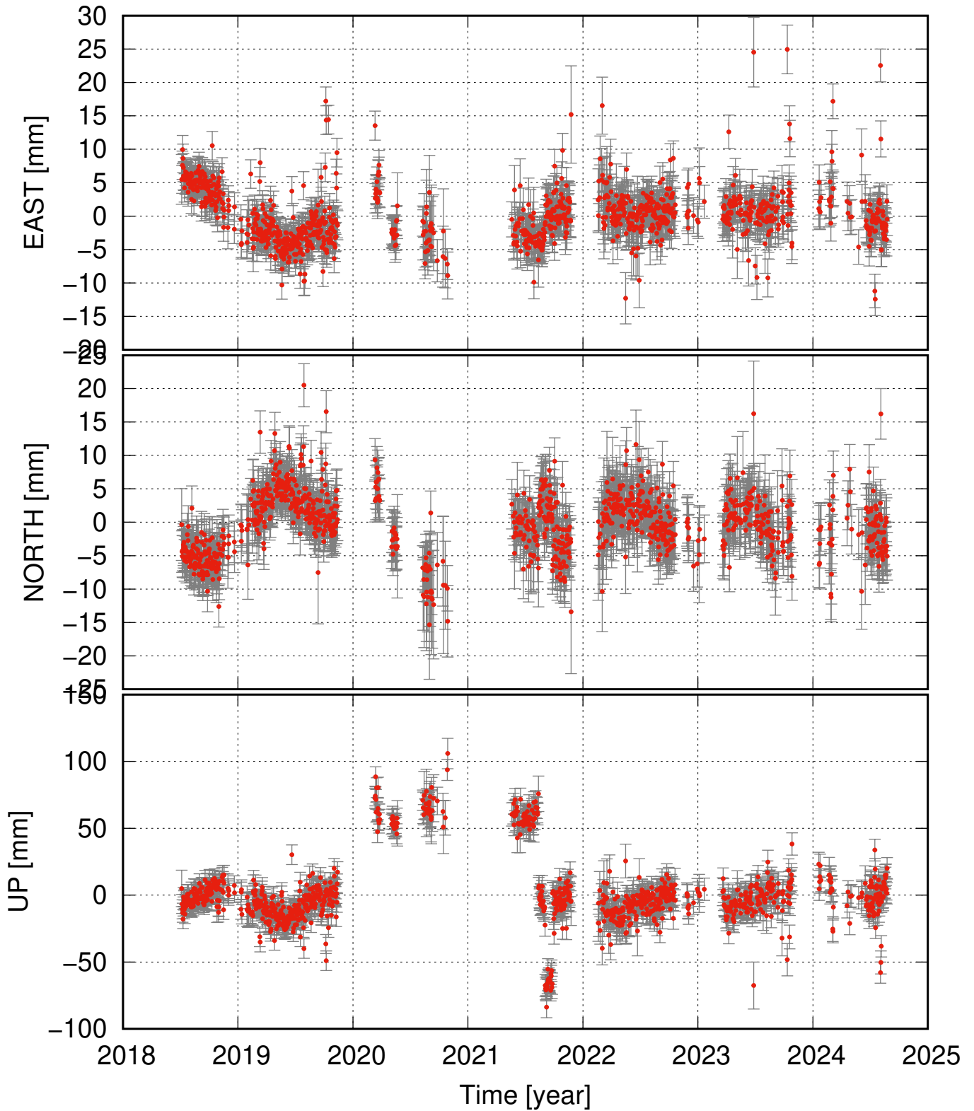
SVIN residual time series (some major events removed as well)
