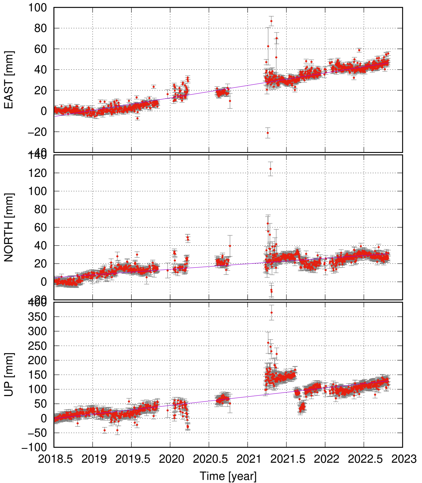
SVIE (64.01, -16.80) time series (ITRF 2014) ve = 12.01 ± 1.13; vn = 6.09 ± 1.53; vu = 30.10 ± 6.74 mm/yr
