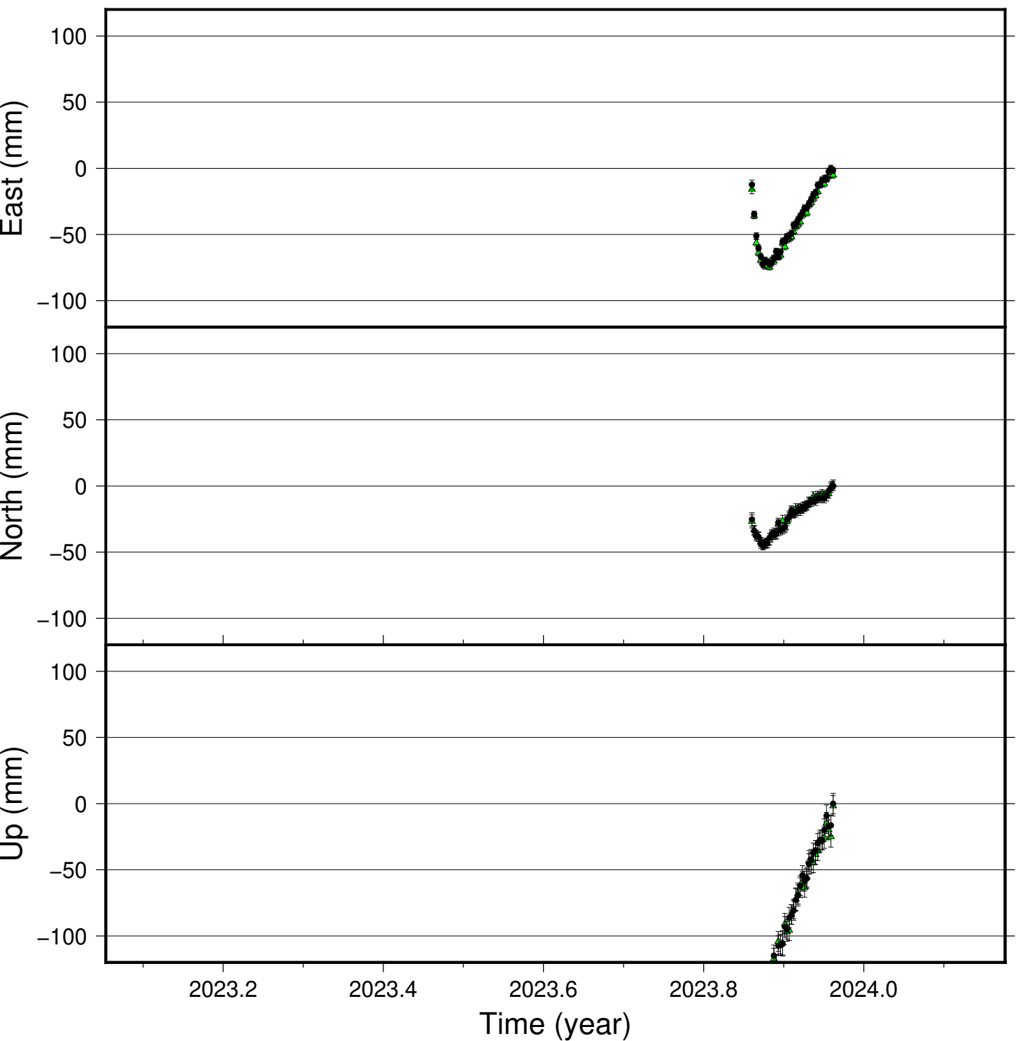
SUND time series (IGS 2014), last 400 days
